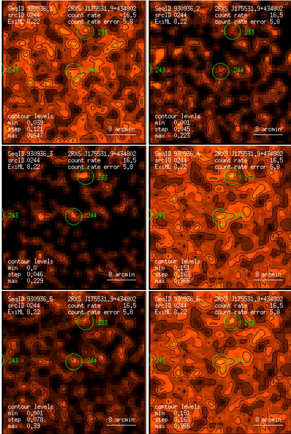
Figure 244: RASS 930936: detection 0244: band rate images, Gaussian filter: (1) PSPC channels 11 – 41, (2) 52 – 90, (3) 91 – 201, (4) 11 – 235, (5) 52 – 201, (6) 11 – 201. Broad band rates in counts/ks. Band rate contour levels in counts/ks/arcmin 2 .
