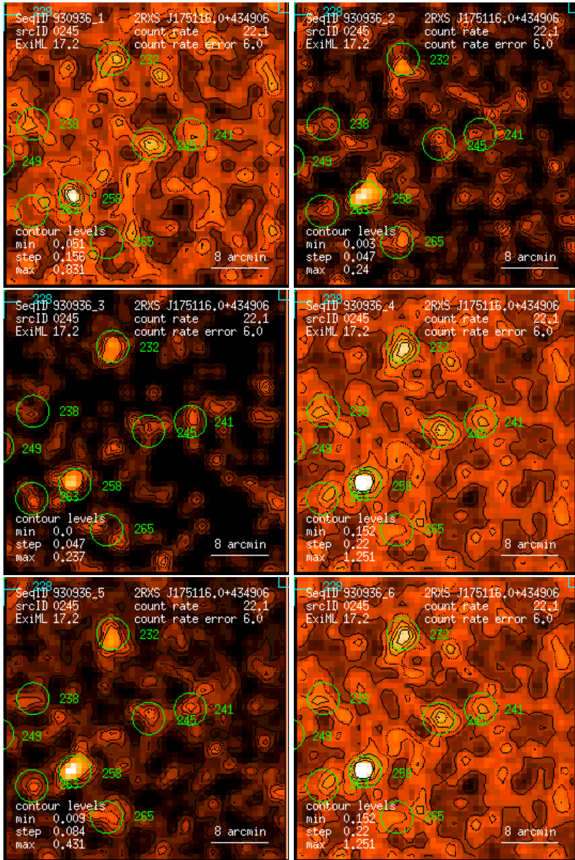
Figure 245: RASS 930936: detection 0245: band rate images, Gaussian filter: (1) PSPC channels 11 – 41, (2) 52 – 90, (3) 91 – 201, (4) 11 – 235, (5) 52 – 201, (6) 11 – 201. Broad band rates in counts/ks. Band rate contour levels in counts/ks/arcmin 2 .
