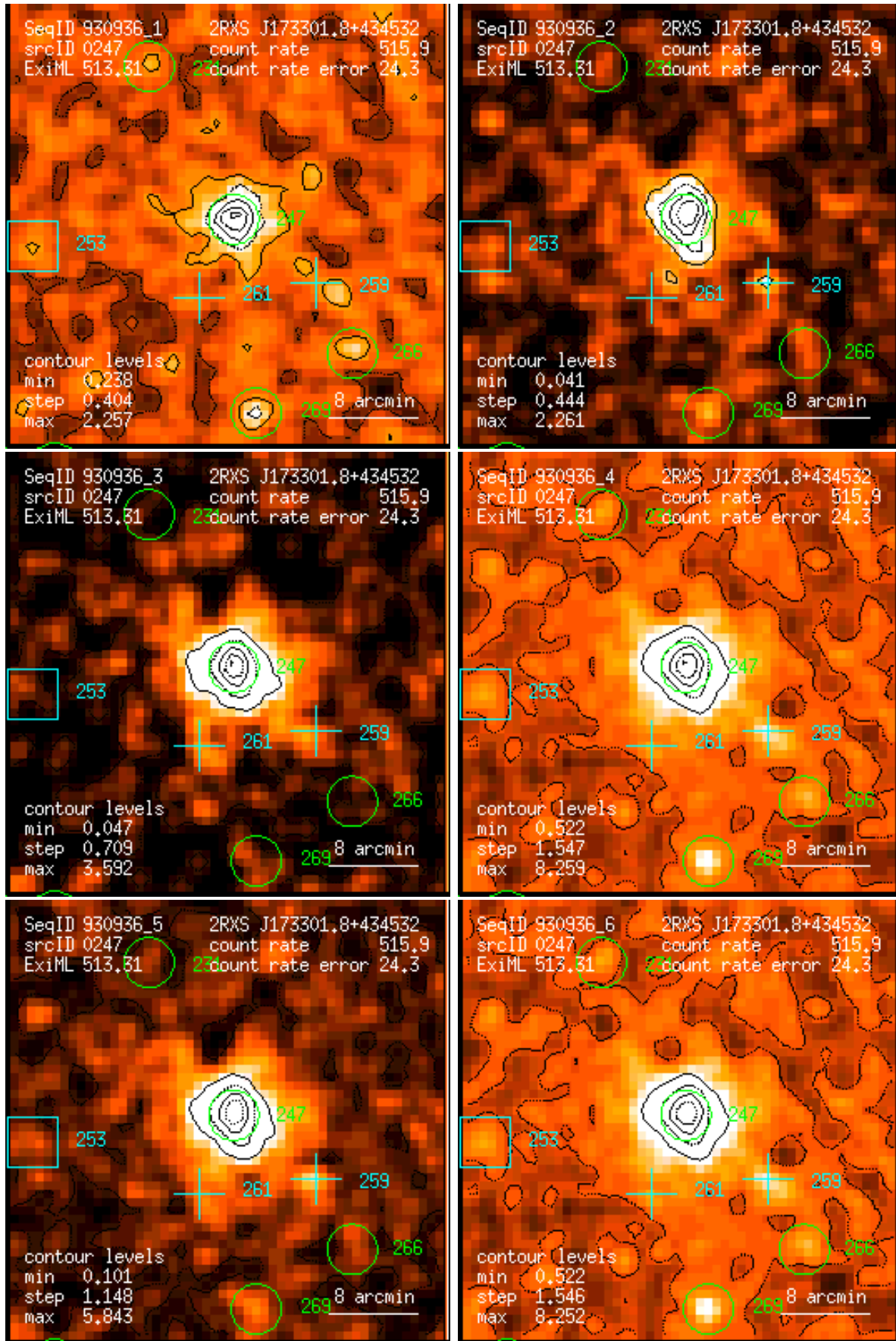
Figure 247: RASS 930936: detection 0247: band rate images, Gaussian filter: (1) PSPC channels 11 – 41, (2) 52 – 90, (3) 91 – 201, (4) 11 – 235, (5) 52 – 201, (6) 11 – 201. Broad band rates in counts/ks. Band rate contour levels in counts/ks/arcmin 2 .
