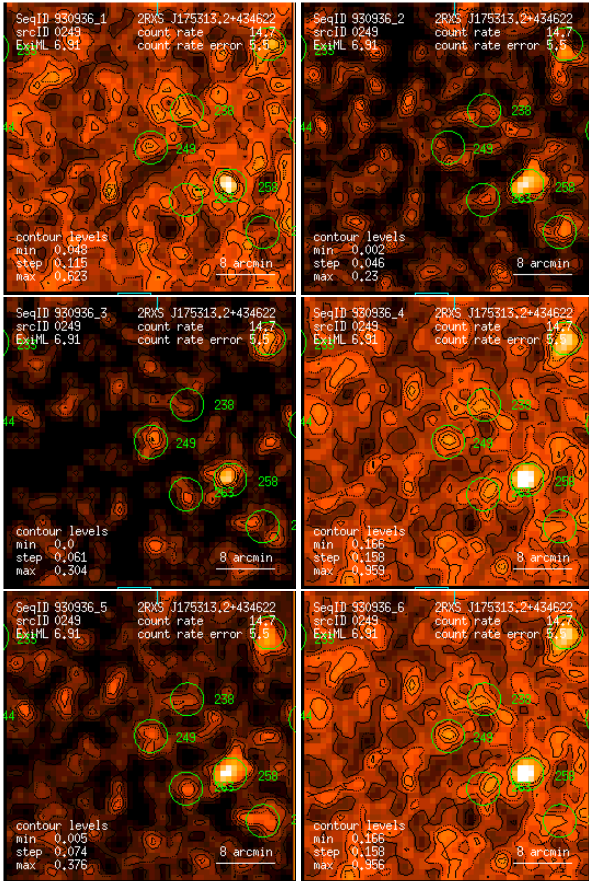
Figure 249: RASS 930936: detection 0249: band rate images, Gaussian filter: (1) PSPC channels 11 – 41, (2) 52 – 90, (3) 91 – 201, (4) 11 – 235, (5) 52 – 201, (6) 11 – 201. Broad band rates in counts/ks. Band rate contour levels in counts/ks/arcmin 2 .
