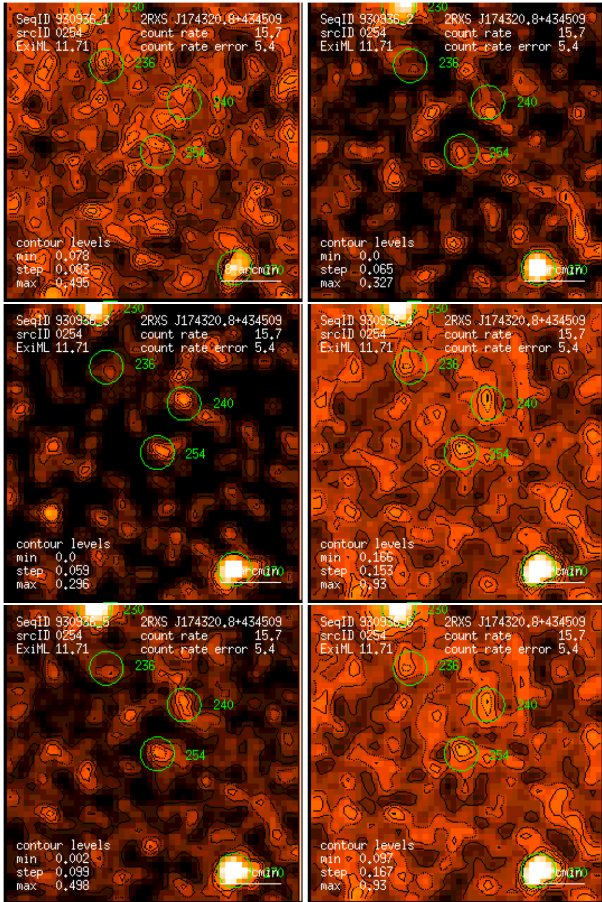
Figure 254: RASS 930936: detection 0254: band rate images, Gaussian filter: (1) PSPC channels 11 – 41, (2) 52 – 90, (3) 91 – 201, (4) 11 – 235, (5) 52 – 201, (6) 11 – 201. Broad band rates in counts/ks. Band rate contour levels in counts/ks/arcmin 2 .
