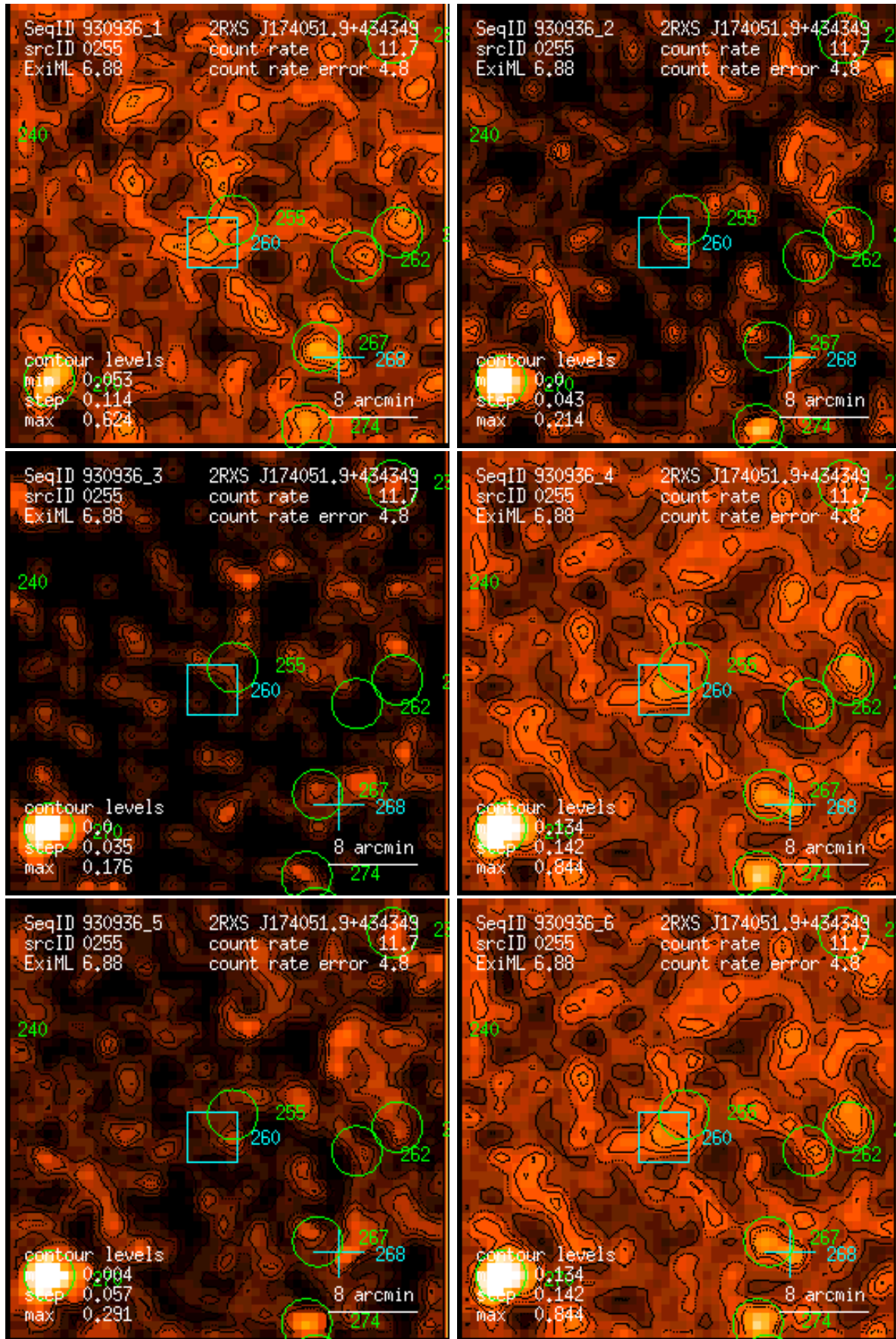
Figure 255: RASS 930936: detection 0255: band rate images, Gaussian filter: (1) PSPC channels 11 – 41, (2) 52 – 90, (3) 91 – 201, (4) 11 – 235, (5) 52 – 201, (6) 11 – 201. Broad band rates in counts/ks. Band rate contour levels in counts/ks/arcmin 2 .
