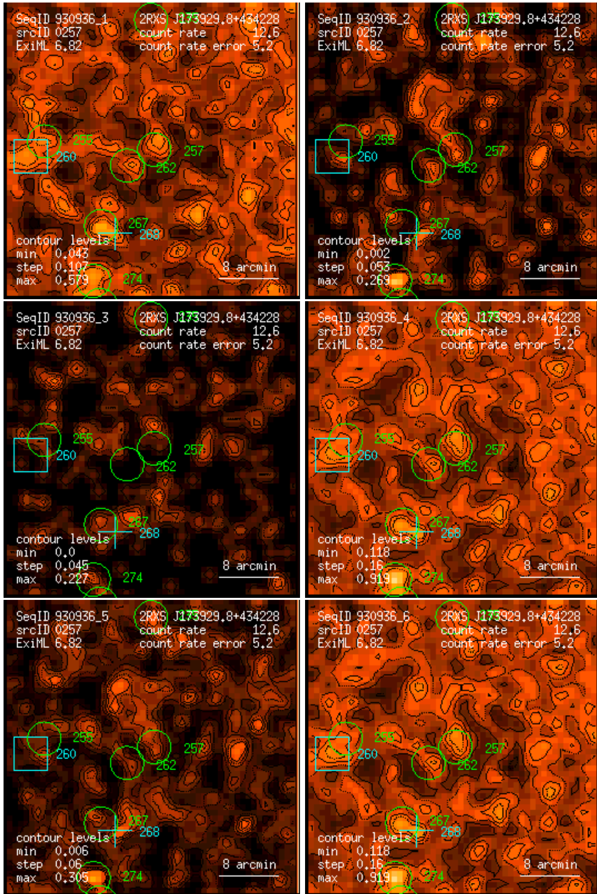
Figure 257: RASS 930936: detection 0257: band rate images, Gaussian filter: (1) PSPC channels 11 – 41, (2) 52 – 90, (3) 91 – 201, (4) 11 – 235, (5) 52 – 201, (6) 11 – 201. Broad band rates in counts/ks. Band rate contour levels in counts/ks/arcmin 2 .
