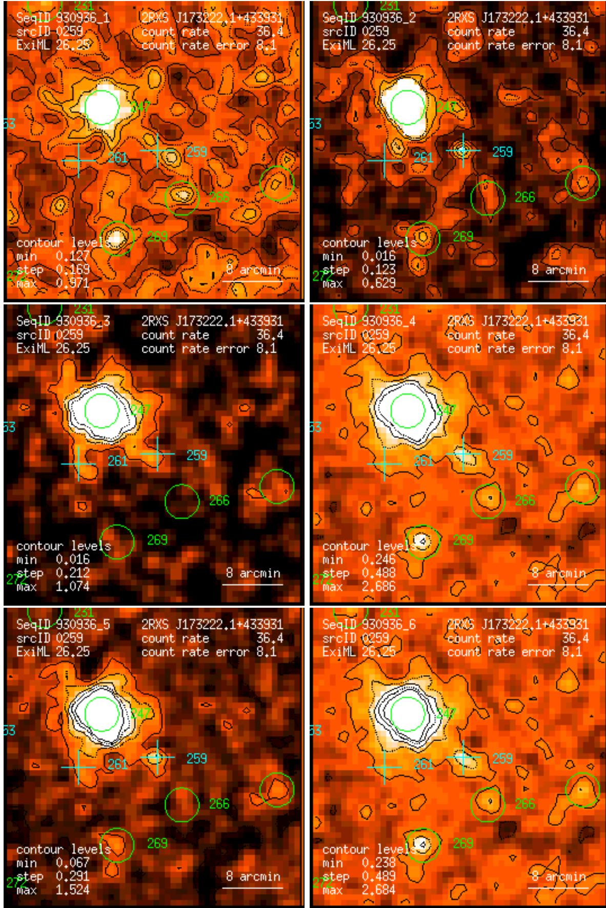
Figure 259: RASS 930936: detection 0259: band rate images, Gaussian filter: (1) PSPC channels 11 – 41, (2) 52 – 90, (3) 91 – 201, (4) 11 – 235, (5) 52 – 201, (6) 11 – 201. Broad band rates in counts/ks. Band rate contour levels in counts/ks/arcmin 2 .
