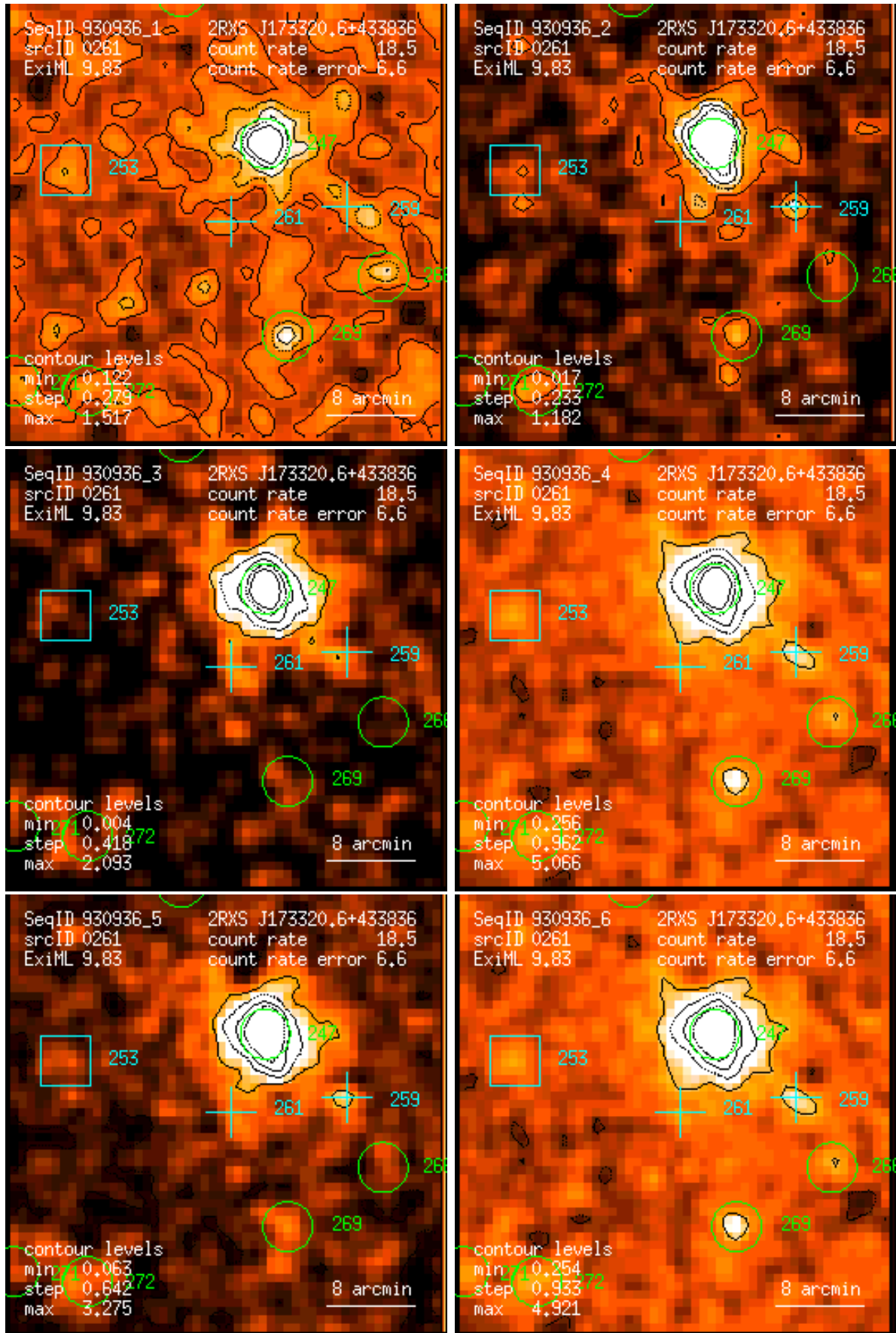
Figure 261: RASS 930936: detection 0261: band rate images, Gaussian filter: (1) PSPC channels 11 – 41, (2) 52 – 90, (3) 91 – 201, (4) 11 – 235, (5) 52 – 201, (6) 11 – 201. Broad band rates in counts/ks. Band rate contour levels in counts/ks/arcmin 2 .
