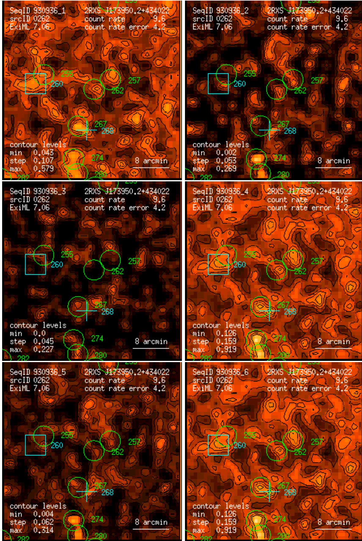
Figure 262: RASS 930936: detection 0262: band rate images, Gaussian filter: (1) PSPC channels 11 – 41, (2) 52 – 90, (3) 91 – 201, (4) 11 – 235, (5) 52 – 201, (6) 11 – 201. Broad band rates in counts/ks. Band rate contour levels in counts/ks/arcmin 2 .
