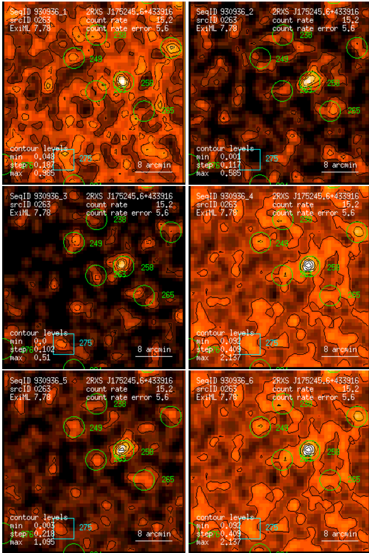
Figure 263: RASS 930936: detection 0263: band rate images, Gaussian filter: (1) PSPC channels 11 – 41, (2) 52 – 90, (3) 91 – 201, (4) 11 – 235, (5) 52 – 201, (6) 11 – 201. Broad band rates in counts/ks. Band rate contour levels in counts/ks/arcmin 2 .
