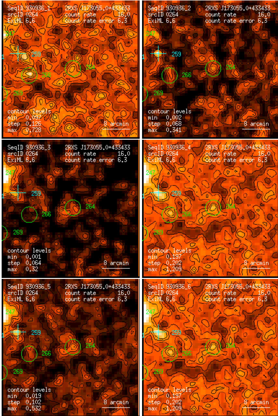
Figure 264: RASS 930936: detection 0264: band rate images, Gaussian filter: (1) PSPC channels 11 – 41, (2) 52 – 90, (3) 91 – 201, (4) 11 – 235, (5) 52 – 201, (6) 11 – 201. Broad band rates in counts/ks. Band rate contour levels in counts/ks/arcmin 2 .
