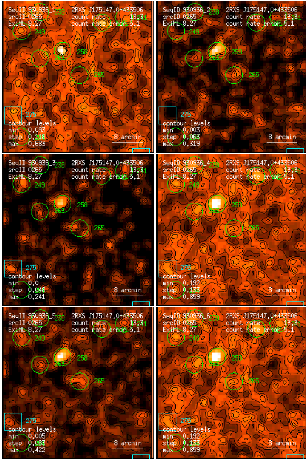
Figure 265: RASS 930936: detection 0265: band rate images, Gaussian filter: (1) PSPC channels 11 – 41, (2) 52 – 90, (3) 91 – 201, (4) 11 – 235, (5) 52 – 201, (6) 11 – 201. Broad band rates in counts/ks. Band rate contour levels in counts/ks/arcmin 2 .
