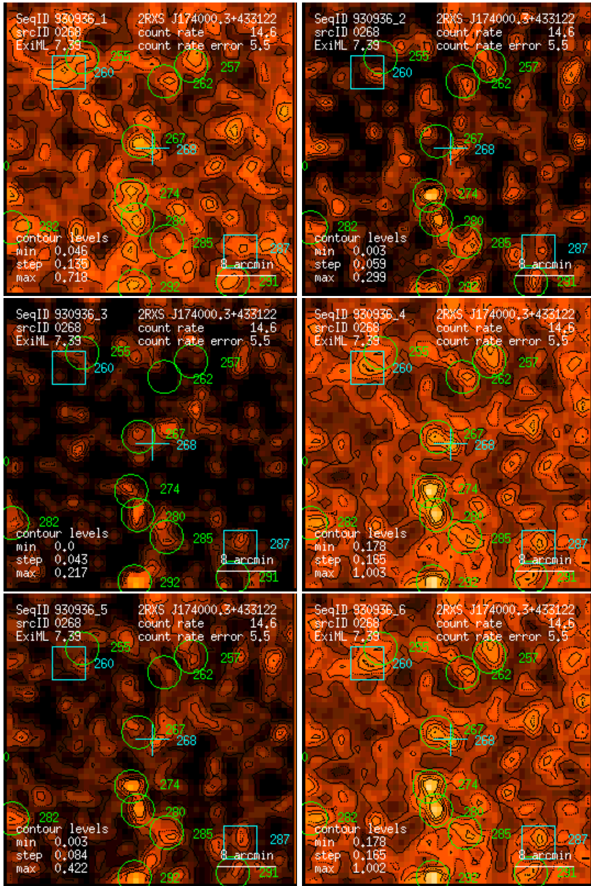
Figure 268: RASS 930936: detection 0268: band rate images, Gaussian filter: (1) PSPC channels 11 – 41, (2) 52 – 90, (3) 91 – 201, (4) 11 – 235, (5) 52 – 201, (6) 11 – 201. Broad band rates in counts/ks. Band rate contour levels in counts/ks/arcmin 2 .
