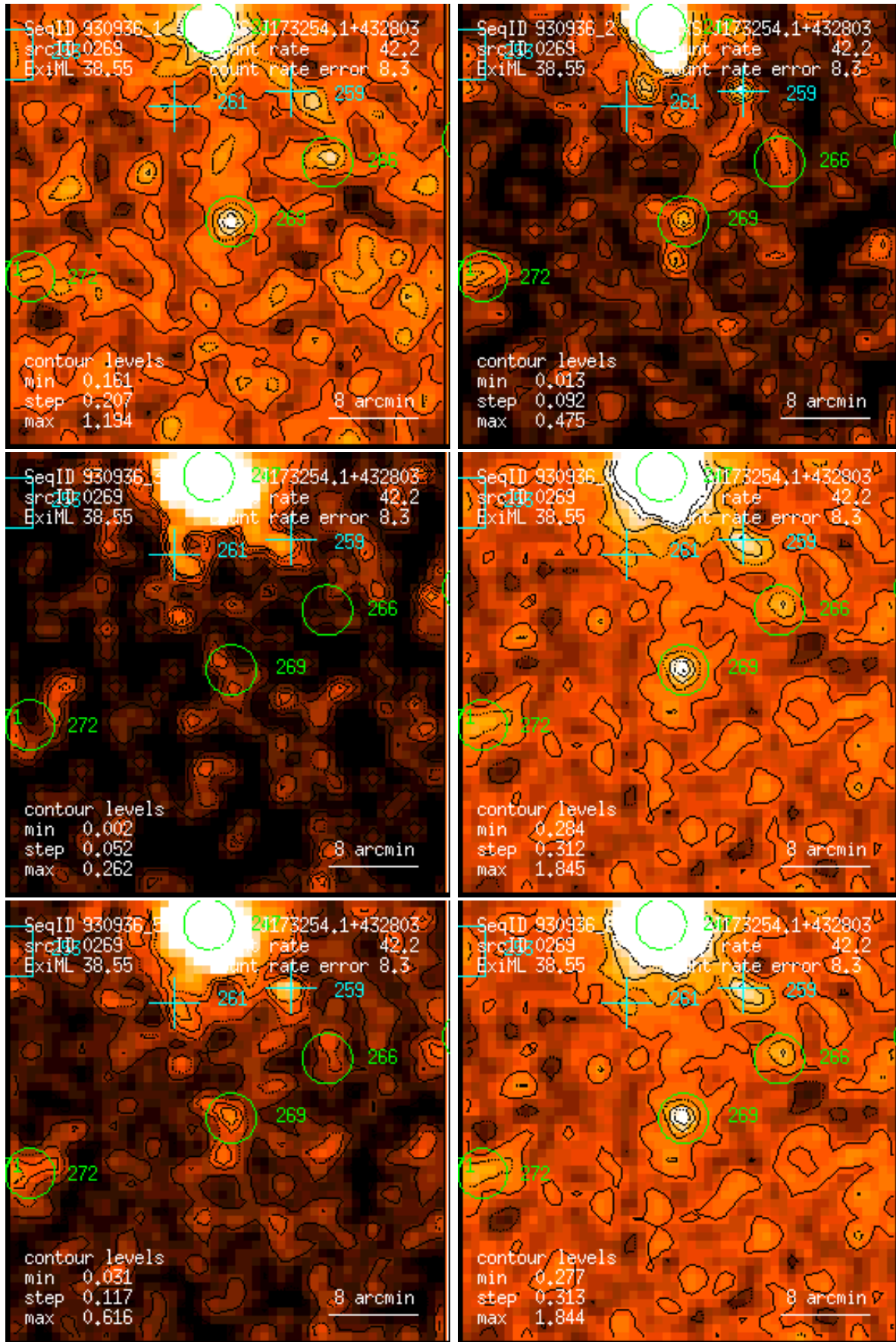
Figure 269: RASS 930936: detection 0269: band rate images, Gaussian filter: (1) PSPC channels 11 – 41, (2) 52 – 90, (3) 91 – 201, (4) 11 – 235, (5) 52 – 201, (6) 11 – 201. Broad band rates in counts/ks. Band rate contour levels in counts/ks/arcmin 2 .
