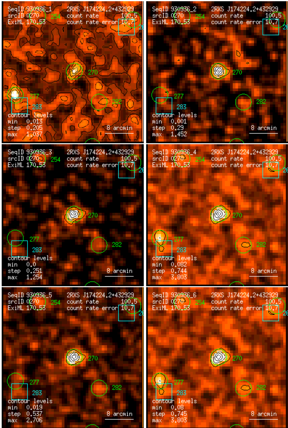
Figure 270: RASS 930936: detection 0270: band rate images, Gaussian filter: (1) PSPC channels 11 – 41, (2) 52 – 90, (3) 91 – 201, (4) 11 – 235, (5) 52 – 201, (6) 11 – 201. Broad band rates in counts/ks. Band rate contour levels in counts/ks/arcmin 2 .
