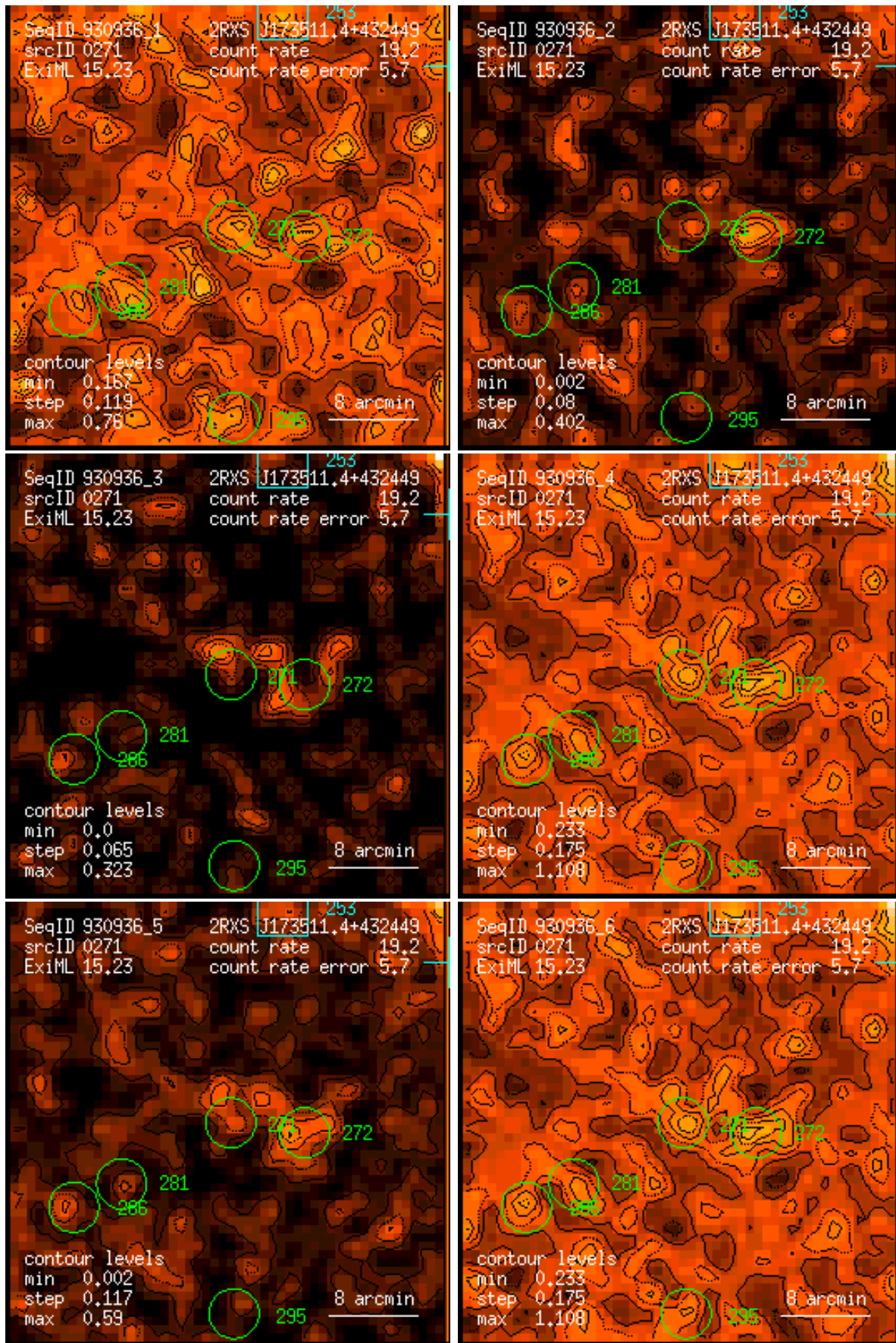
Figure 271: RASS 930936: detection 0271: band rate images, Gaussian filter: (1) PSPC channels 11 – 41, (2) 52 – 90, (3) 91 – 201, (4) 11 – 235, (5) 52 – 201, (6) 11 – 201. Broad band rates in counts/ks. Band rate contour levels in counts/ks/arcmin 2 .
