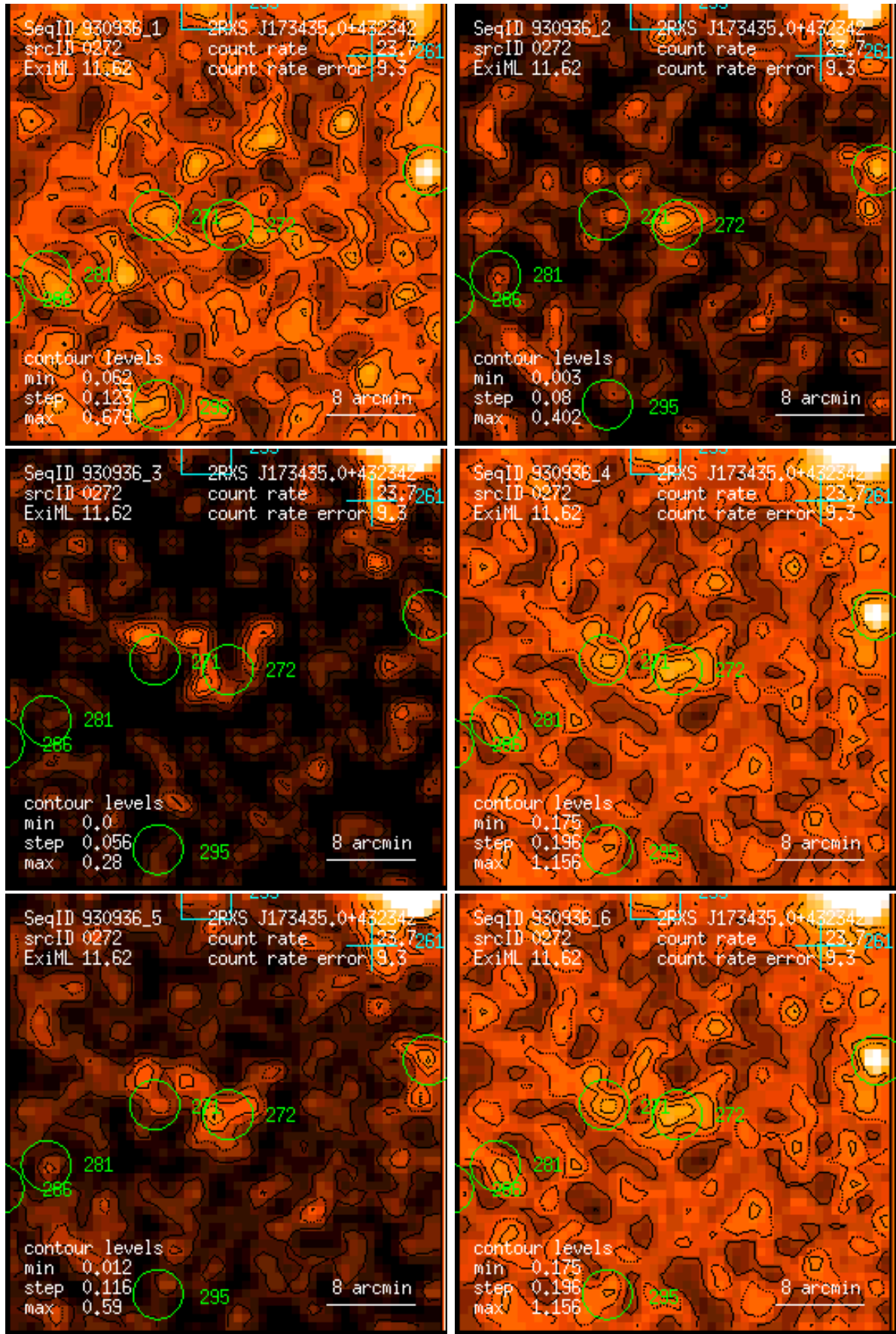
Figure 272: RASS 930936: detection 0272: band rate images, Gaussian filter: (1) PSPC channels 11 – 41, (2) 52 – 90, (3) 91 – 201, (4) 11 – 235, (5) 52 – 201, (6) 11 – 201. Broad band rates in counts/ks. Band rate contour levels in counts/ks/arcmin 2 .
