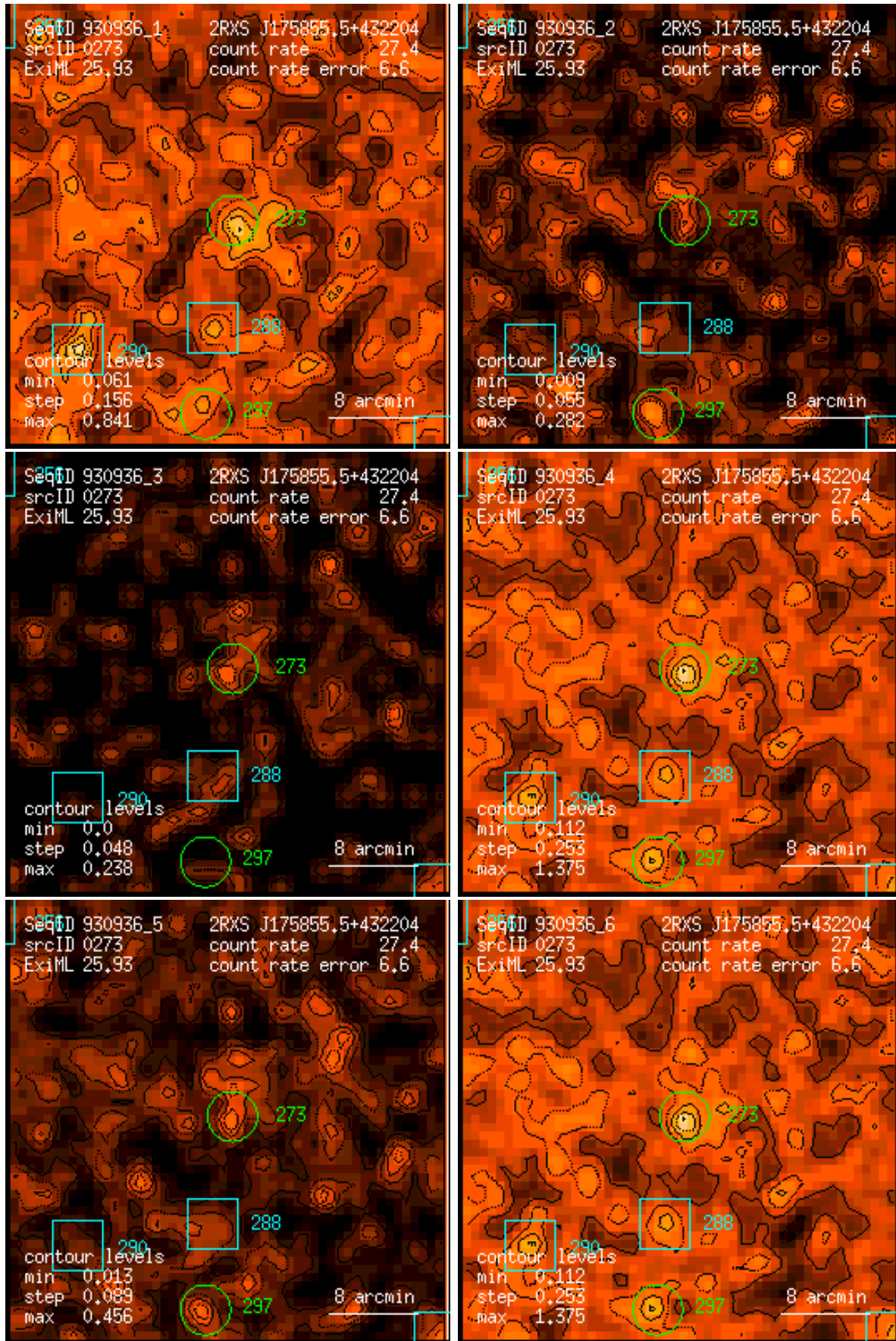
Figure 273: RASS 930936: detection 0273: band rate images, Gaussian filter: (1) PSPC channels 11 – 41, (2) 52 – 90, (3) 91 – 201, (4) 11 – 235, (5) 52 – 201, (6) 11 – 201. Broad band rates in counts/ks. Band rate contour levels in counts/ks/arcmin 2 .
