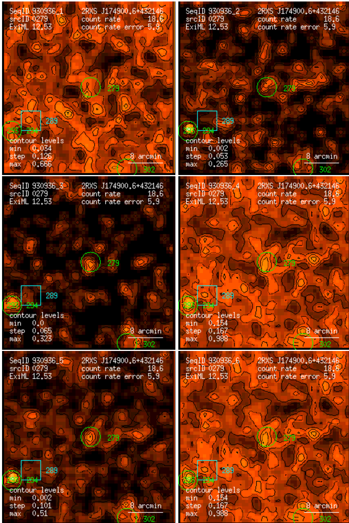
Figure 279: RASS 930936: detection 0279: band rate images, Gaussian filter: (1) PSPC channels 11 – 41, (2) 52 – 90, (3) 91 – 201, (4) 11 – 235, (5) 52 – 201, (6) 11 – 201. Broad band rates in counts/ks. Band rate contour levels in counts/ks/arcmin 2 .
