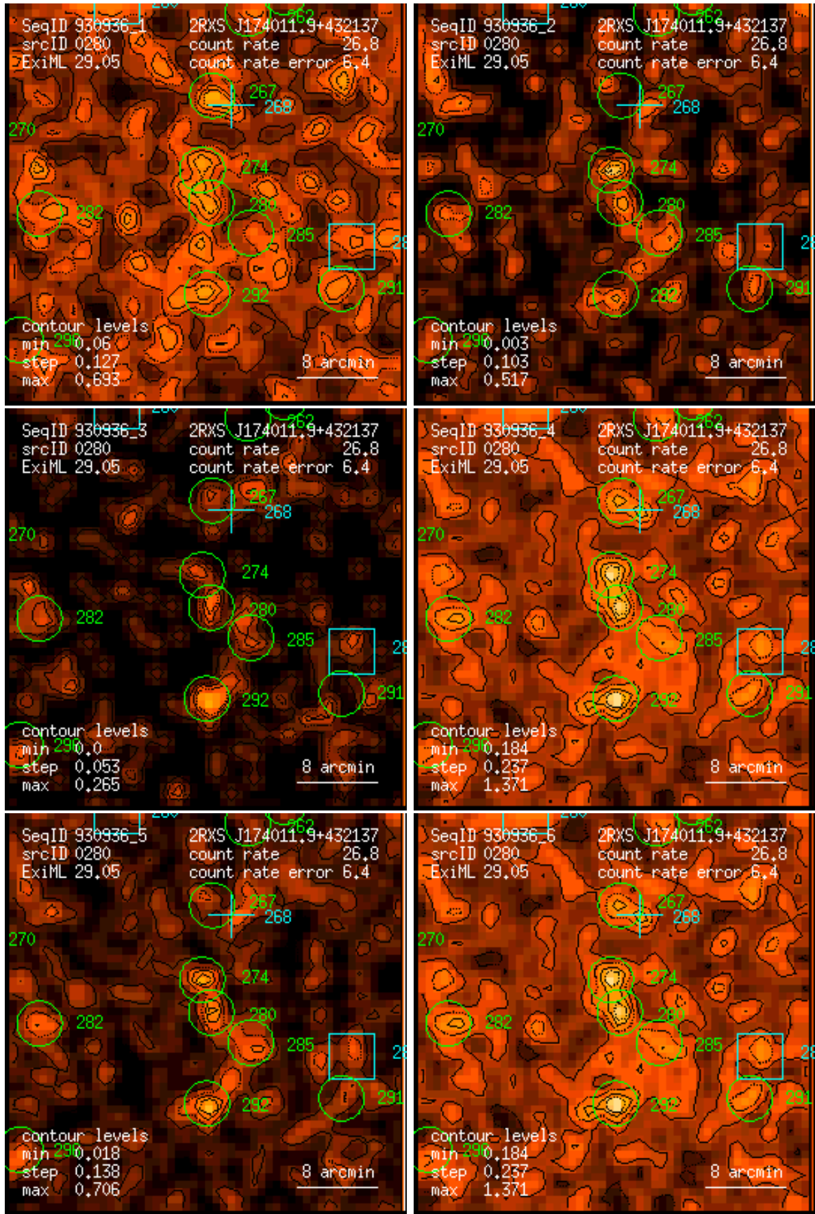
Figure 280: RASS 930936: detection 0280: band rate images, Gaussian filter: (1) PSPC channels 11 – 41, (2) 52 – 90, (3) 91 – 201, (4) 11 – 235, (5) 52 – 201, (6) 11 – 201. Broad band rates in counts/ks. Band rate contour levels in counts/ks/arcmin 2 .
