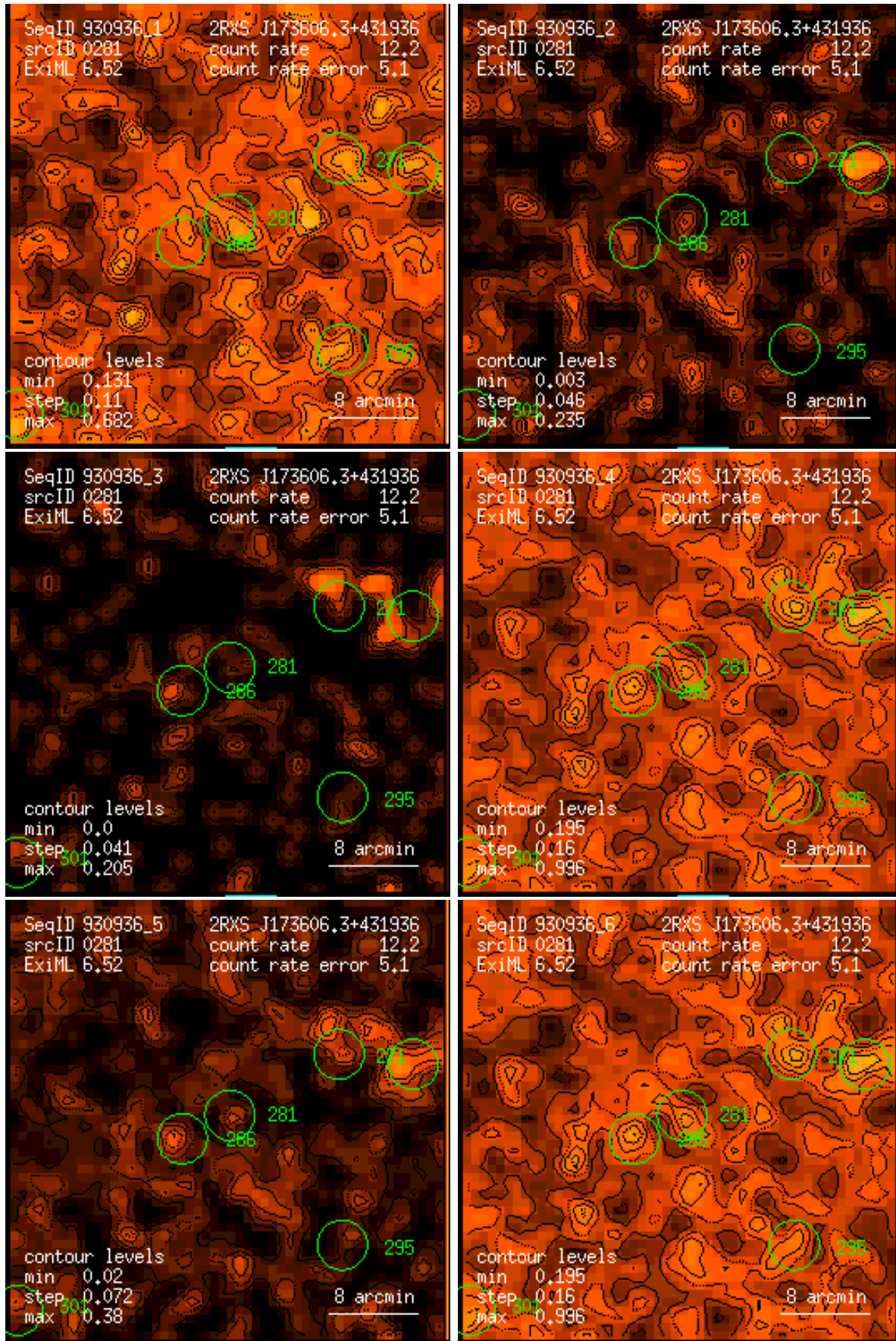
Figure 281: RASS 930936: detection 0281: band rate images, Gaussian filter: (1) PSPC channels 11 – 41, (2) 52 – 90, (3) 91 – 201, (4) 11 – 235, (5) 52 – 201, (6) 11 – 201. Broad band rates in counts/ks. Band rate contour levels in counts/ks/arcmin 2 .
