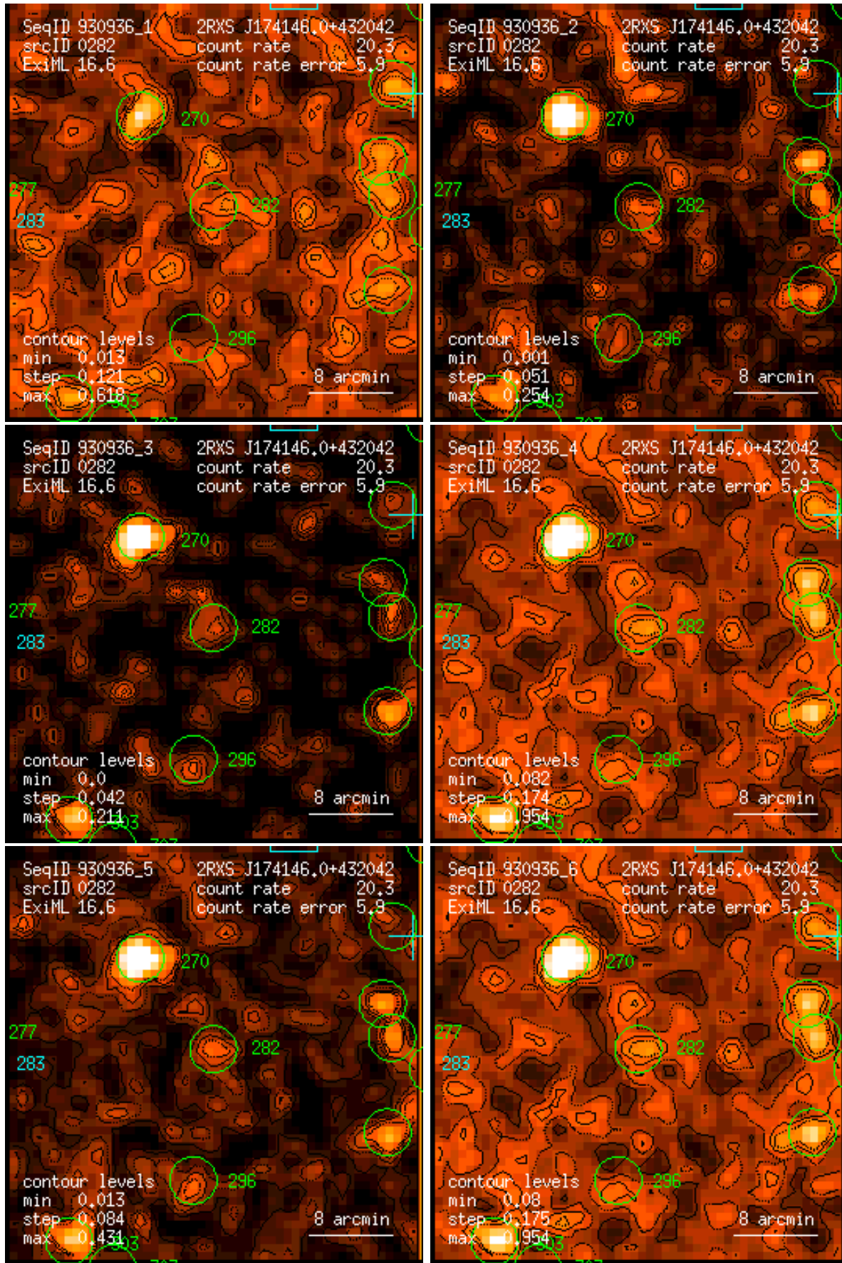
Figure 282: RASS 930936: detection 0282: band rate images, Gaussian filter: (1) PSPC channels 11 – 41, (2) 52 – 90, (3) 91 – 201, (4) 11 – 235, (5) 52 – 201, (6) 11 – 201. Broad band rates in counts/ks. Band rate contour levels in counts/ks/arcmin 2 .
