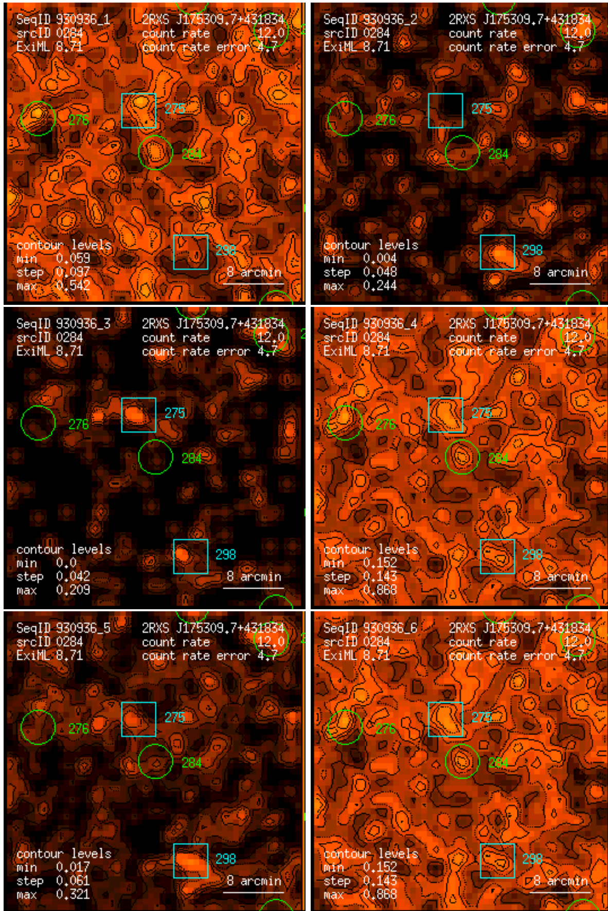
Figure 284: RASS 930936: detection 0284: band rate images, Gaussian filter: (1) PSPC channels 11 – 41, (2) 52 – 90, (3) 91 – 201, (4) 11 – 235, (5) 52 – 201, (6) 11 – 201. Broad band rates in counts/ks. Band rate contour levels in counts/ks/arcmin 2 .
