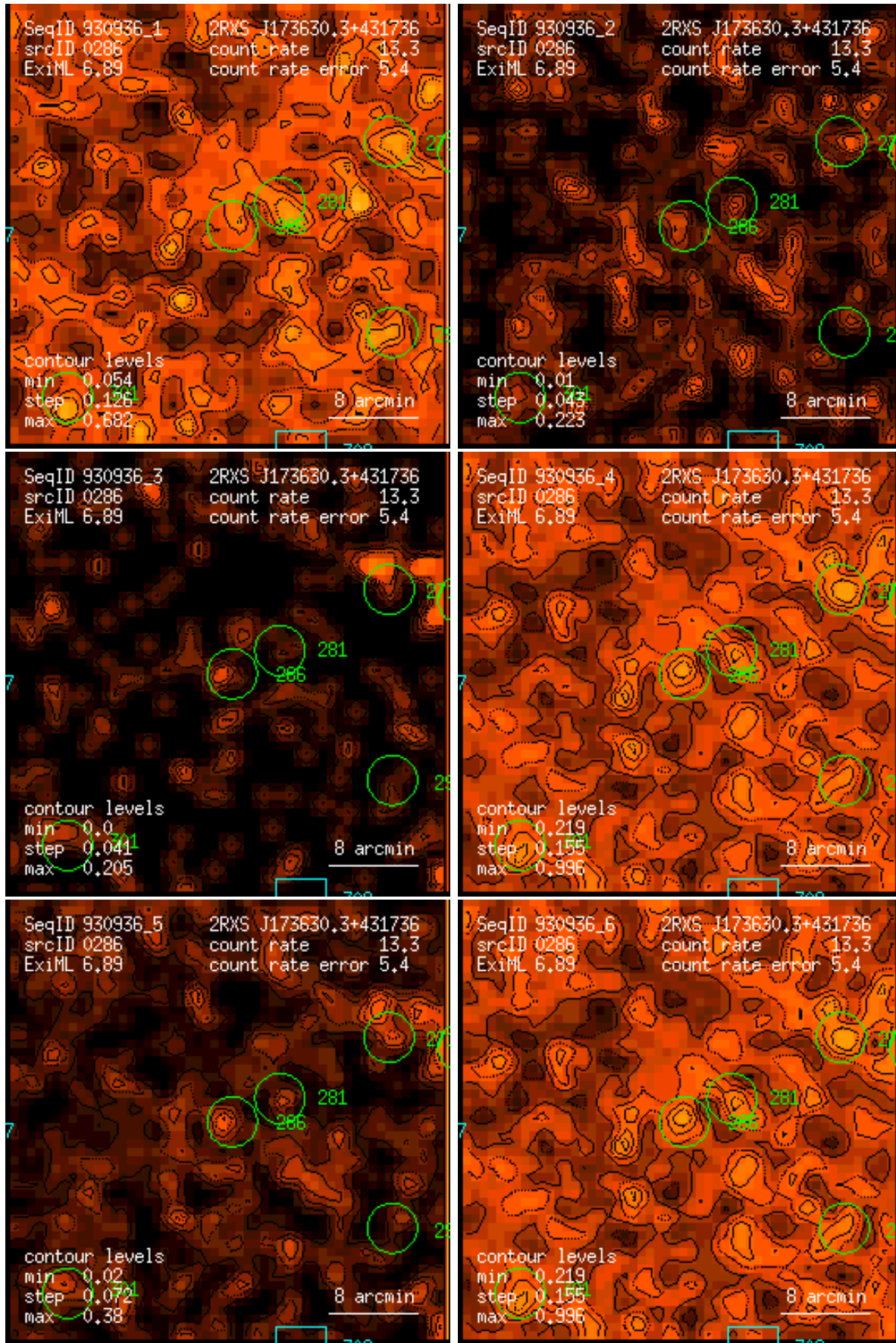
Figure 286: RASS 930936: detection 0286: band rate images, Gaussian filter: (1) PSPC channels 11 – 41, (2) 52 – 90, (3) 91 – 201, (4) 11 – 235, (5) 52 – 201, (6) 11 – 201. Broad band rates in counts/ks. Band rate contour levels in counts/ks/arcmin 2 .
