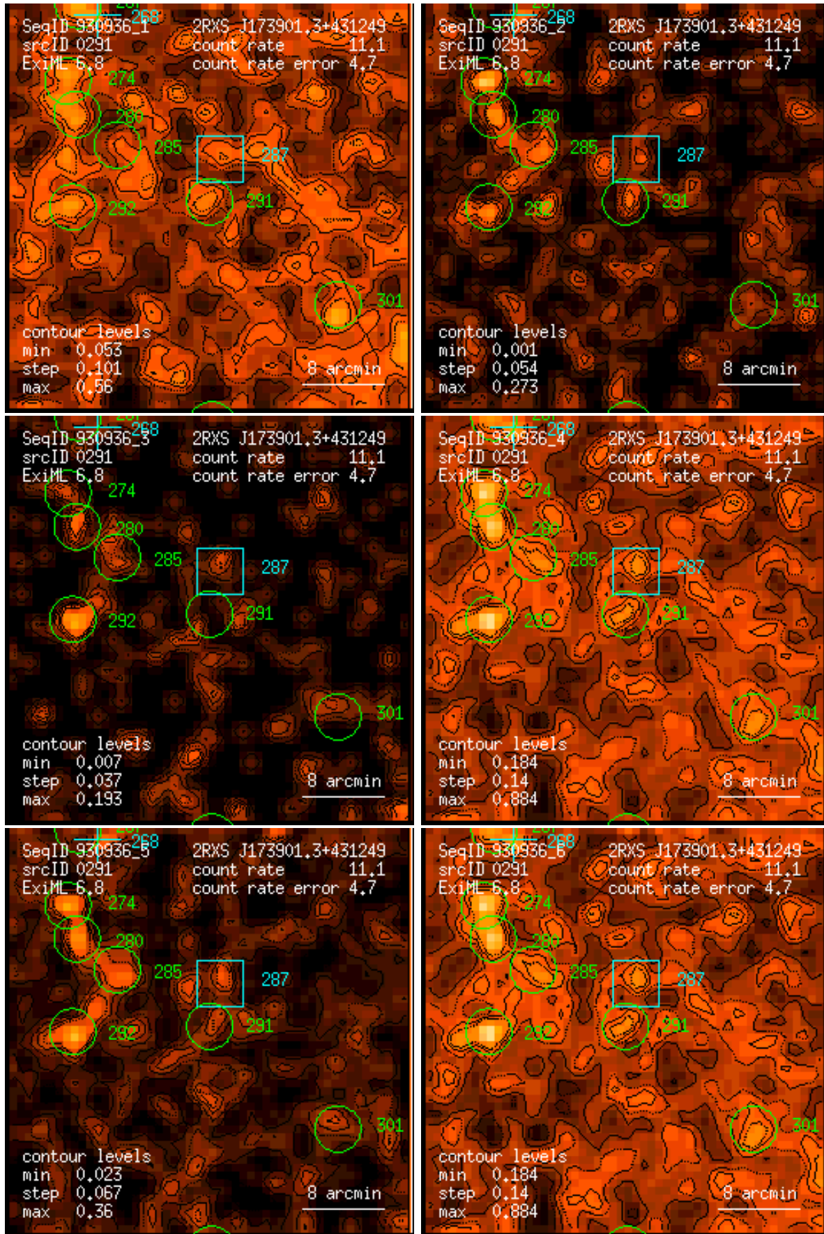
Figure 291: RASS 930936: detection 0291: band rate images, Gaussian filter: (1) PSPC channels 11 – 41, (2) 52 – 90, (3) 91 – 201, (4) 11 – 235, (5) 52 – 201, (6) 11 – 201. Broad band rates in counts/ks. Band rate contour levels in counts/ks/arcmin 2 .
