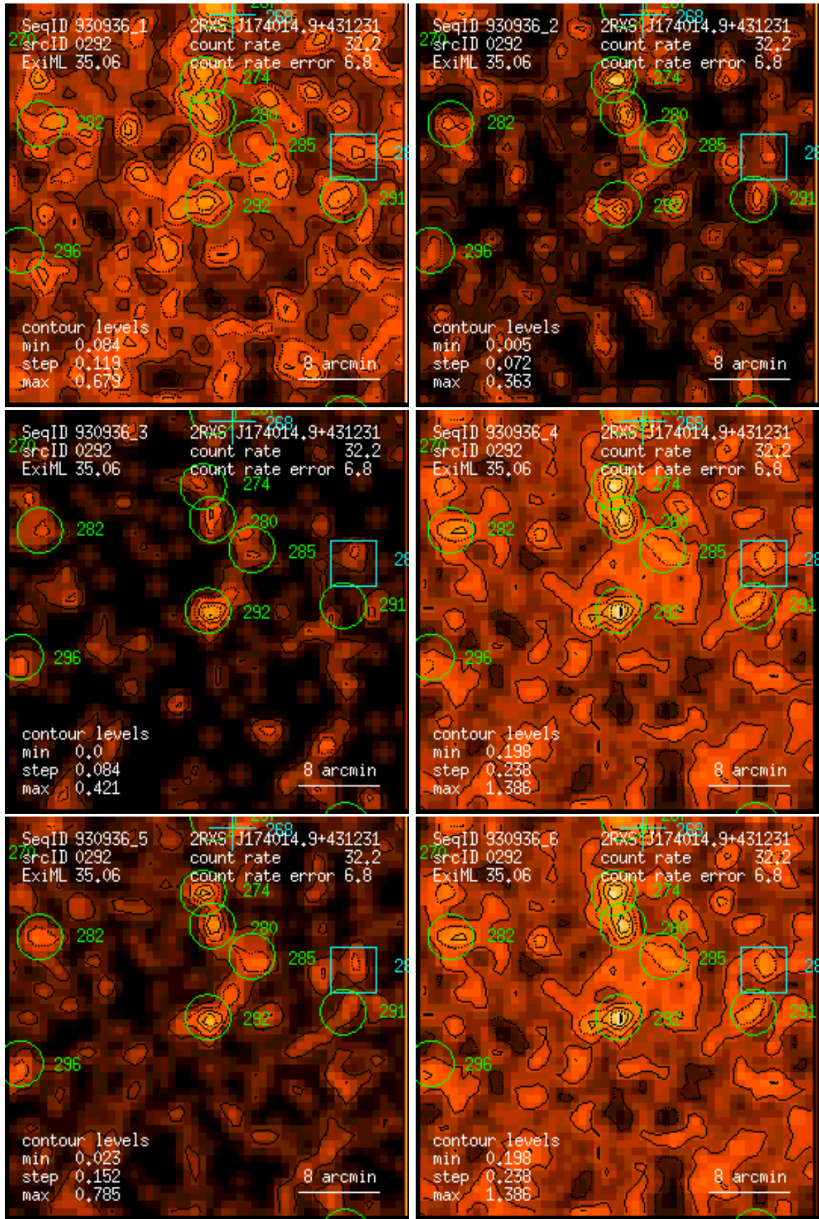
Figure 292: RASS 930936: detection 0292: band rate images, Gaussian filter: (1) PSPC channels 11 – 41, (2) 52 – 90, (3) 91 – 201, (4) 11 – 235, (5) 52 – 201, (6) 11 – 201. Broad band rates in counts/ks. Band rate contour levels in counts/ks/arcmin 2 .
