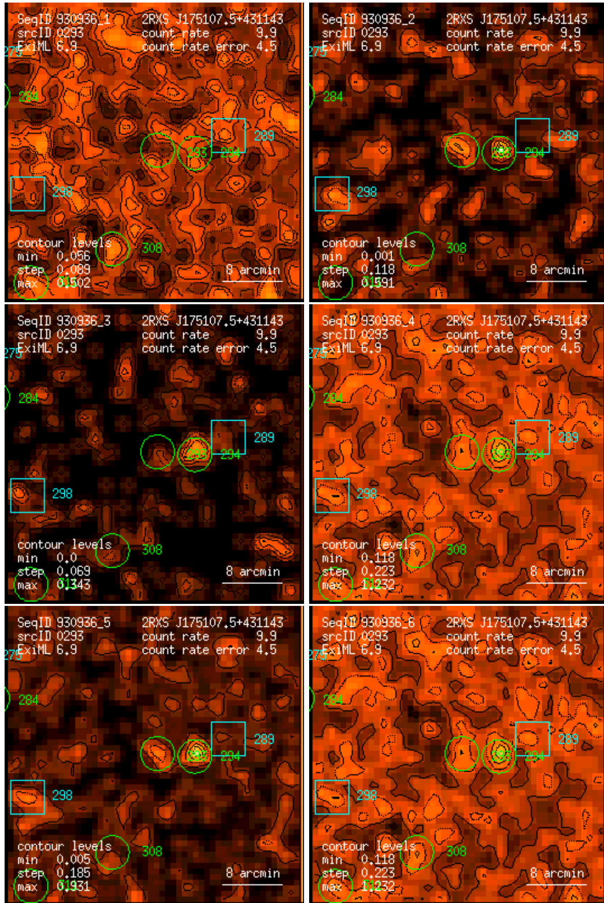
Figure 293: RASS 930936: detection 0293: band rate images, Gaussian filter: (1) PSPC channels 11 – 41, (2) 52 – 90, (3) 91 – 201, (4) 11 – 235, (5) 52 – 201, (6) 11 – 201. Broad band rates in counts/ks. Band rate contour levels in counts/ks/arcmin 2 .
