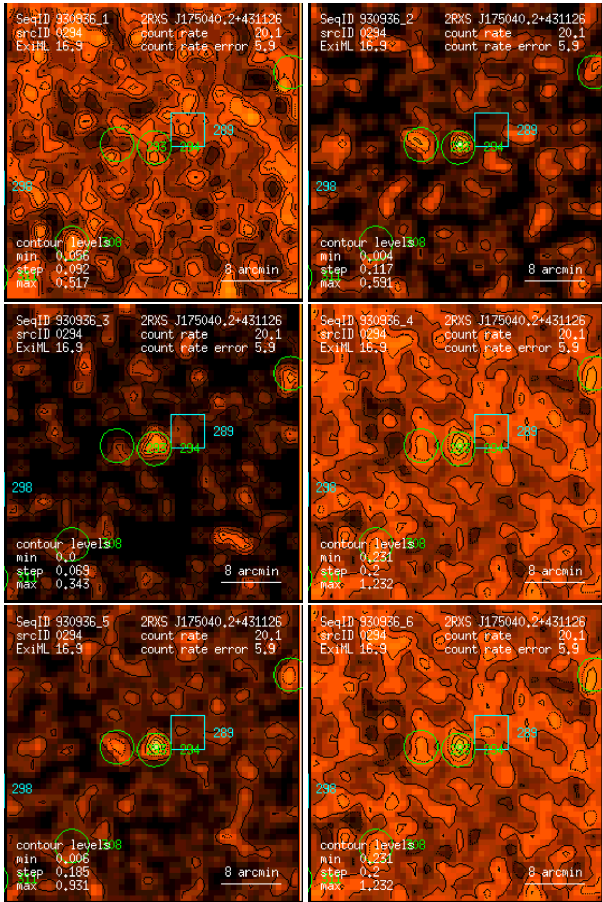
Figure 294: RASS 930936: detection 0294: band rate images, Gaussian filter: (1) PSPC channels 11 – 41, (2) 52 – 90, (3) 91 – 201, (4) 11 – 235, (5) 52 – 201, (6) 11 – 201. Broad band rates in counts/ks. Band rate contour levels in counts/ks/arcmin 2 .
