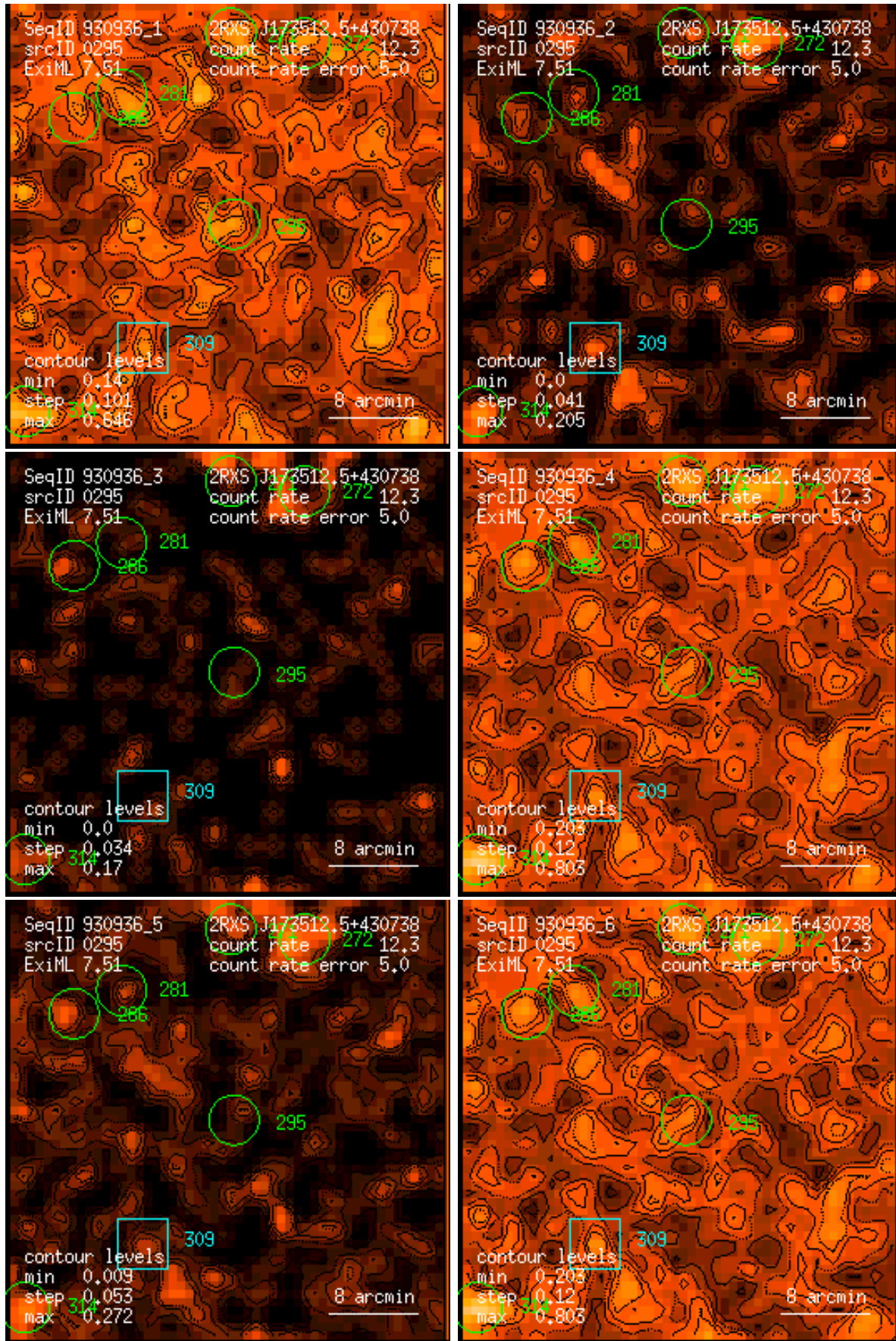
Figure 295: RASS 930936: detection 0295: band rate images, Gaussian filter: (1) PSPC channels 11 – 41, (2) 52 – 90, (3) 91 – 201, (4) 11 – 235, (5) 52 – 201, (6) 11 – 201. Broad band rates in counts/ks. Band rate contour levels in counts/ks/arcmin 2 .
