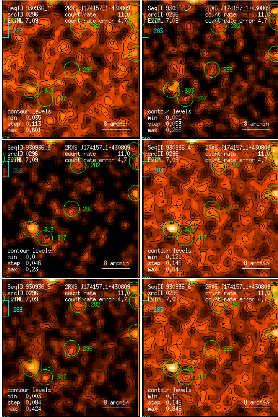
Figure 296: RASS 930936: detection 0296: band rate images, Gaussian filter: (1) PSPC channels 11 – 41, (2) 52 – 90, (3) 91 – 201, (4) 11 – 235, (5) 52 – 201, (6) 11 – 201. Broad band rates in counts/ks. Band rate contour levels in counts/ks/arcmin 2 .
