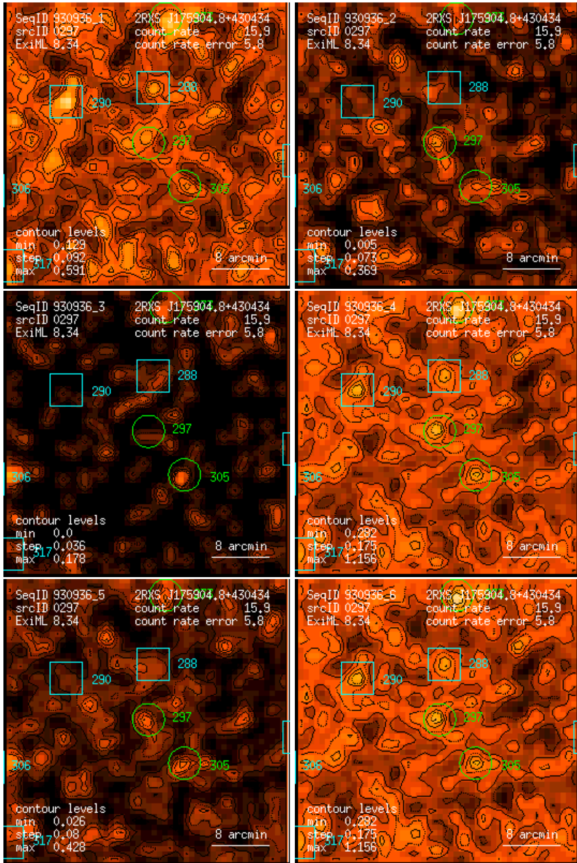
Figure 297: RASS 930936: detection 0297: band rate images, Gaussian filter: (1) PSPC channels 11 – 41, (2) 52 – 90, (3) 91 – 201, (4) 11 – 235, (5) 52 – 201, (6) 11 – 201. Broad band rates in counts/ks. Band rate contour levels in counts/ks/arcmin 2 .
