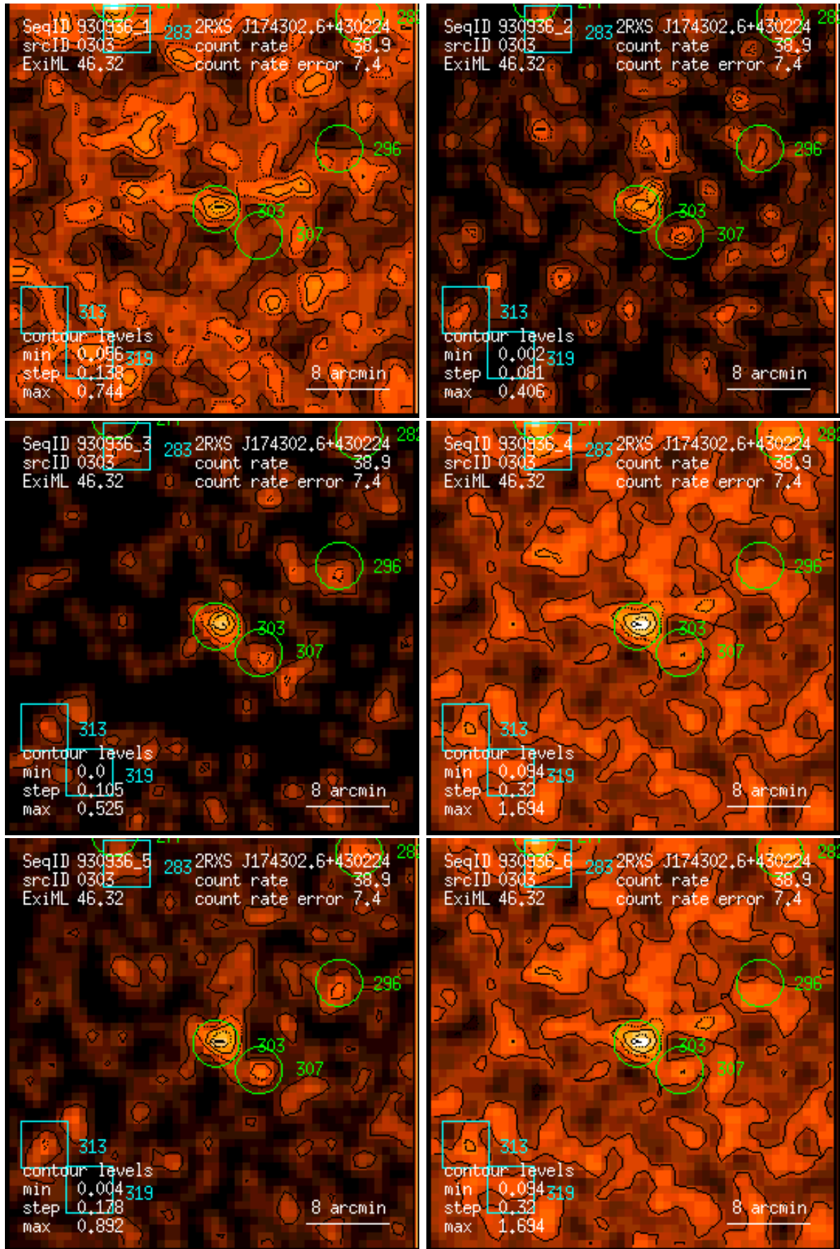
Figure 303: RASS 930936: detection 0303: band rate images, Gaussian filter: (1) PSPC channels 11 – 41, (2) 52 – 90, (3) 91 – 201, (4) 11 – 235, (5) 52 – 201, (6) 11 – 201. Broad band rates in counts/ks. Band rate contour levels in counts/ks/arcmin 2 .
