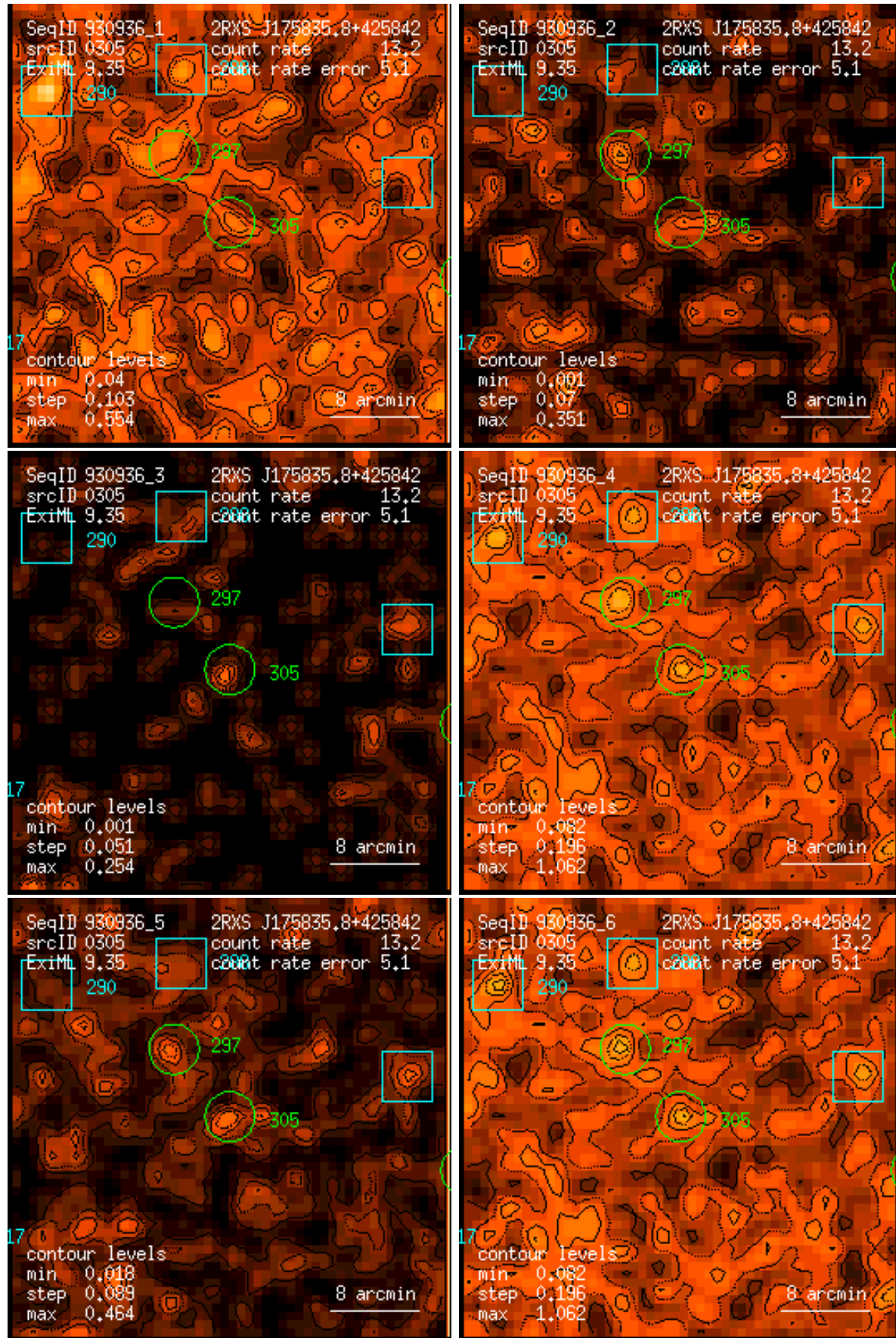
Figure 305: RASS 930936: detection 0305: band rate images, Gaussian filter: (1) PSPC channels 11 – 41, (2) 52 – 90, (3) 91 – 201, (4) 11 – 235, (5) 52 – 201, (6) 11 – 201. Broad band rates in counts/ks. Band rate contour levels in counts/ks/arcmin 2 .
