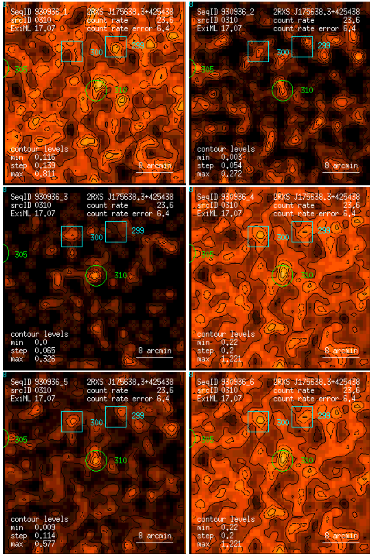
Figure 310: RASS 930936: detection 0310: band rate images, Gaussian filter: (1) PSPC channels 11 – 41, (2) 52 – 90, (3) 91 – 201, (4) 11 – 235, (5) 52 – 201, (6) 11 – 201. Broad band rates in counts/ks. Band rate contour levels in counts/ks/arcmin 2 .
