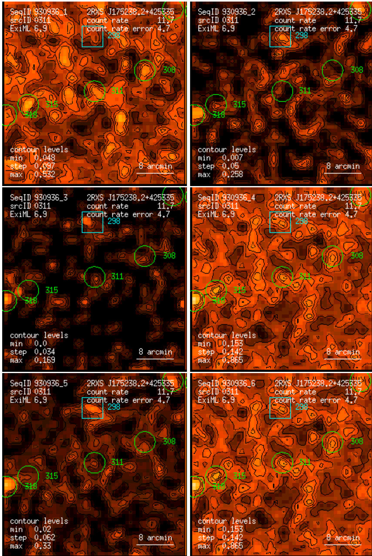
Figure 311: RASS 930936: detection 0311: band rate images, Gaussian filter: (1) PSPC channels 11 – 41, (2) 52 – 90, (3) 91 – 201, (4) 11 – 235, (5) 52 – 201, (6) 11 – 201. Broad band rates in counts/ks. Band rate contour levels in counts/ks/arcmin 2 .
