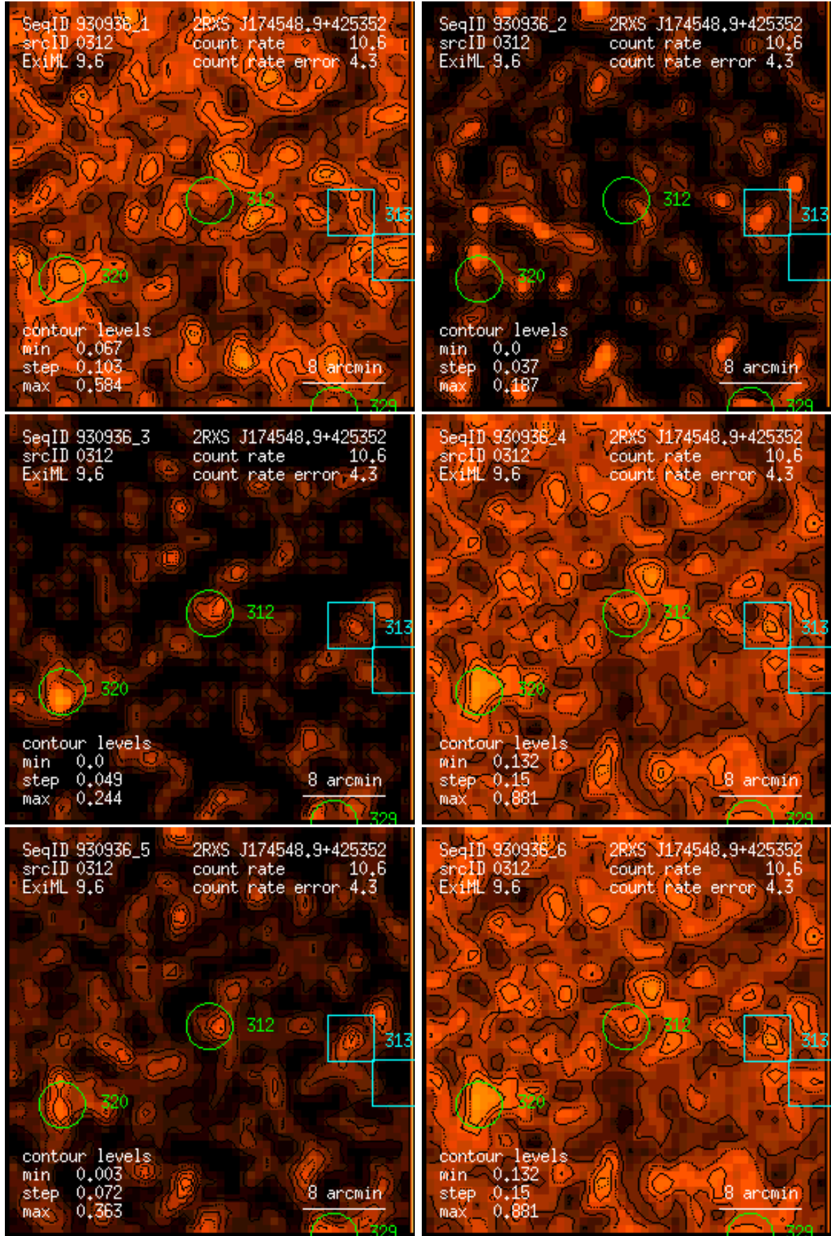
Figure 312: RASS 930936: detection 0312: band rate images, Gaussian filter: (1) PSPC channels 11 – 41, (2) 52 – 90, (3) 91 – 201, (4) 11 – 235, (5) 52 – 201, (6) 11 – 201. Broad band rates in counts/ks. Band rate contour levels in counts/ks/arcmin 2 .
