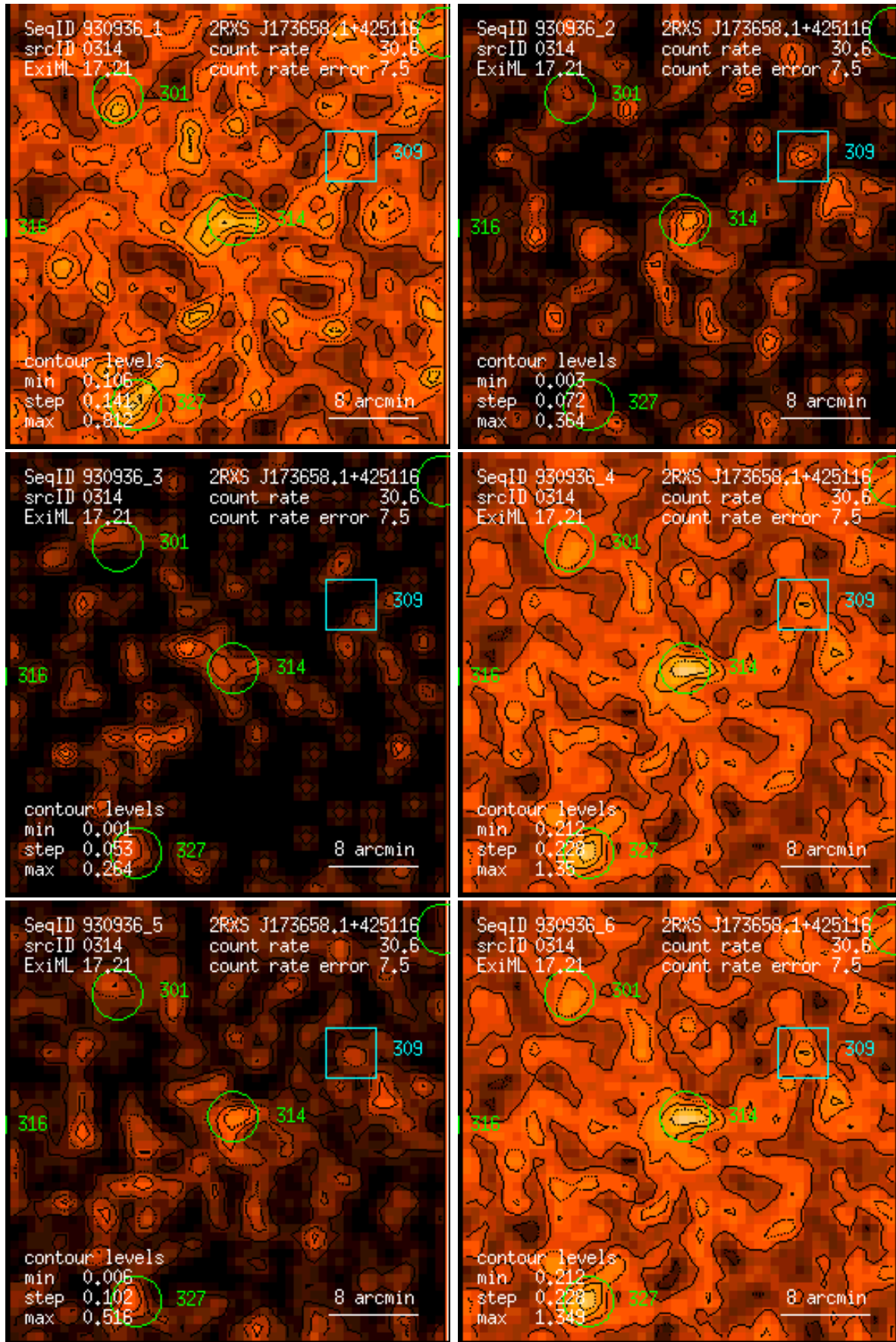
Figure 314: RASS 930936: detection 0314: band rate images, Gaussian filter: (1) PSPC channels 11 – 41, (2) 52 – 90, (3) 91 – 201, (4) 11 – 235, (5) 52 – 201, (6) 11 – 201. Broad band rates in counts/ks. Band rate contour levels in counts/ks/arcmin 2 .
