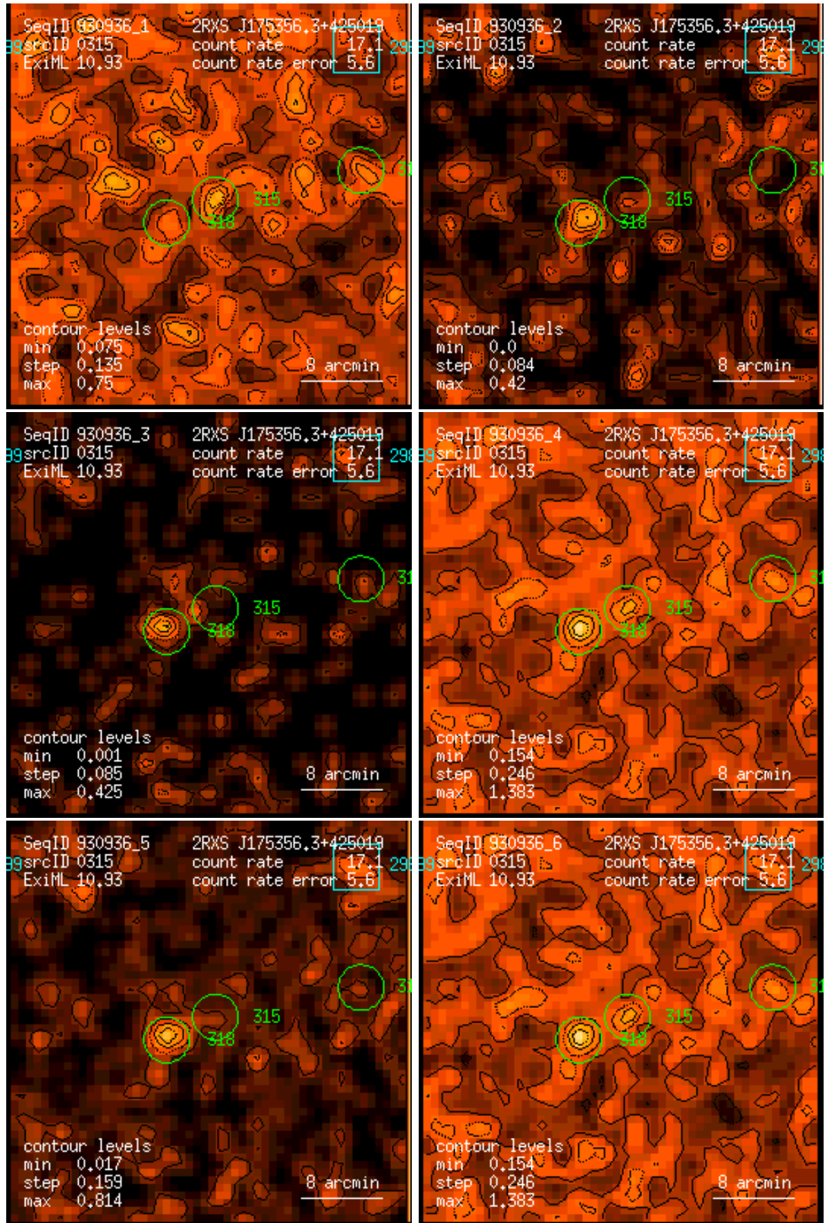
Figure 315: RASS 930936: detection 0315: band rate images, Gaussian filter: (1) PSPC channels 11 – 41, (2) 52 – 90, (3) 91 – 201, (4) 11 – 235, (5) 52 – 201, (6) 11 – 201. Broad band rates in counts/ks. Band rate contour levels in counts/ks/arcmin 2 .
