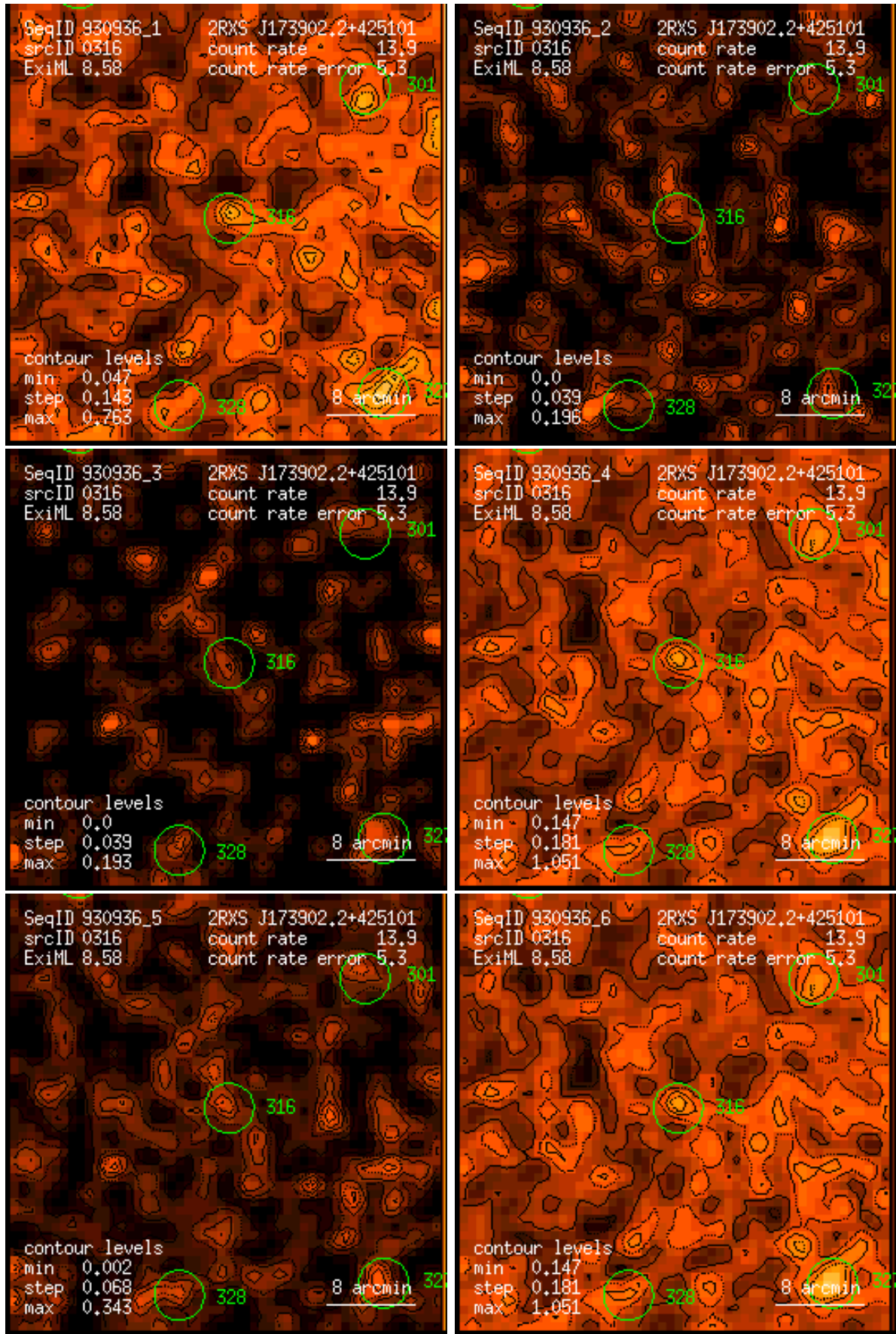
Figure 316: RASS 930936: detection 0316: band rate images, Gaussian filter: (1) PSPC channels 11 – 41, (2) 52 – 90, (3) 91 – 201, (4) 11 – 235, (5) 52 – 201, (6) 11 – 201. Broad band rates in counts/ks. Band rate contour levels in counts/ks/arcmin 2 .
