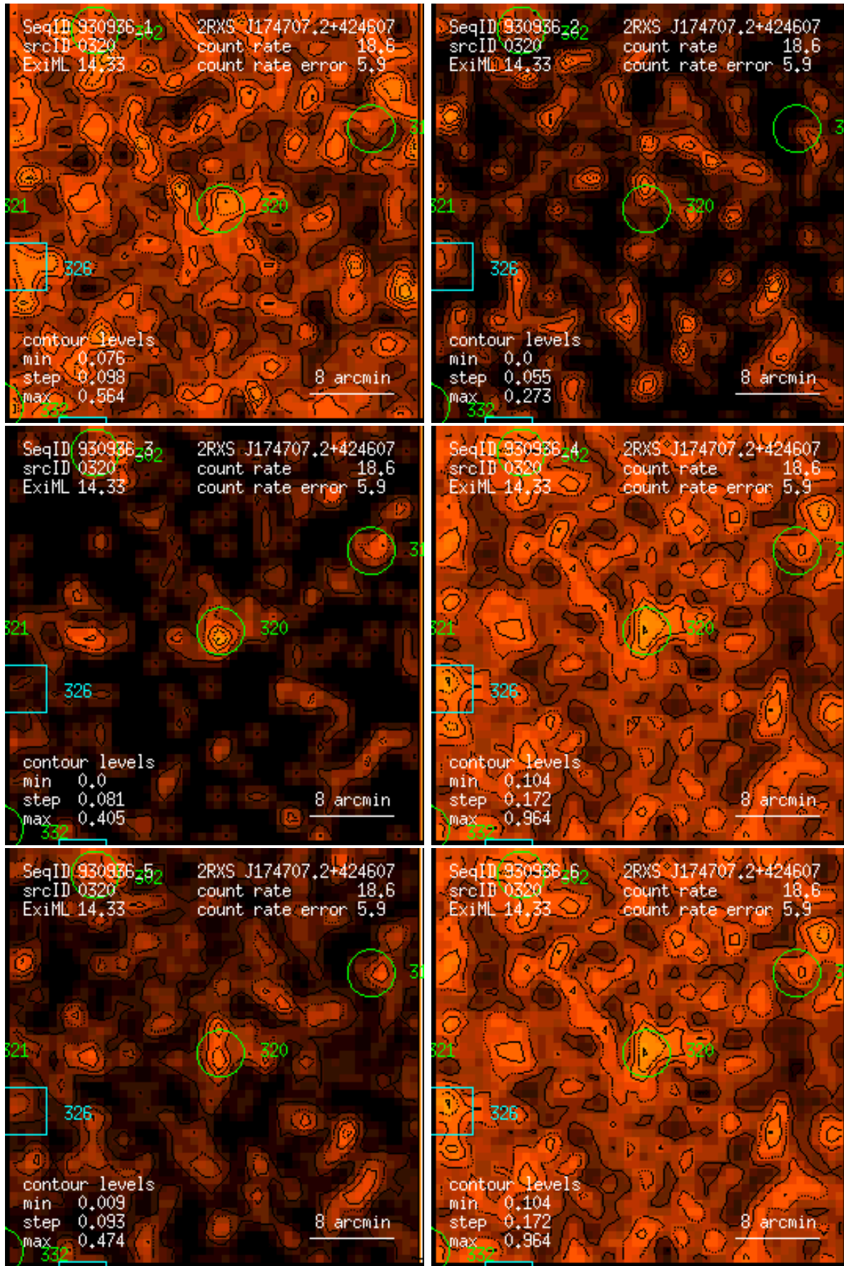
Figure 320: RASS 930936: detection 0320: band rate images, Gaussian filter: (1) PSPC channels 11 – 41, (2) 52 – 90, (3) 91 – 201, (4) 11 – 235, (5) 52 – 201, (6) 11 – 201. Broad band rates in counts/ks. Band rate contour levels in counts/ks/arcmin 2 .
