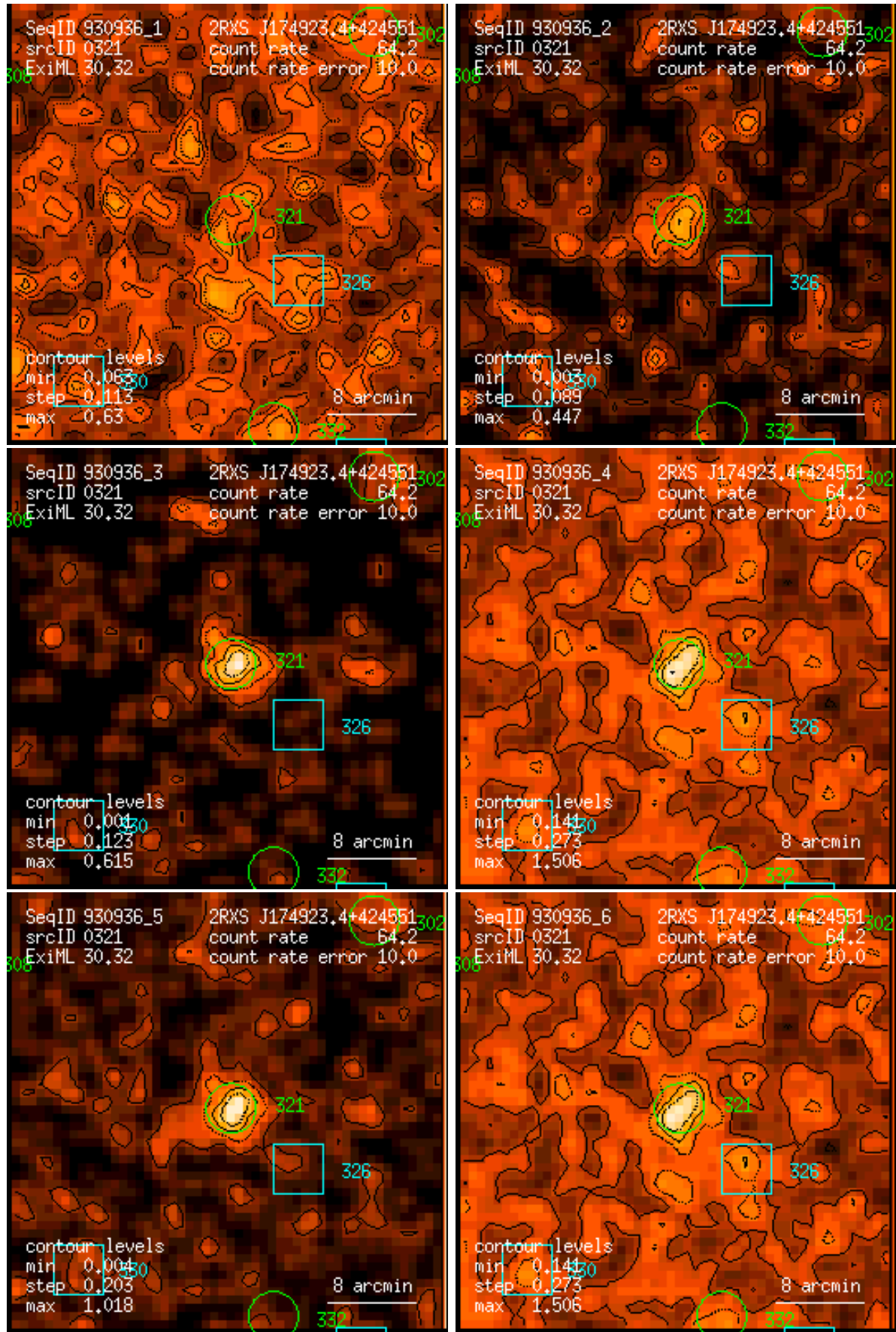
Figure 321: RASS 930936: detection 0321: band rate images, Gaussian filter: (1) PSPC channels 11 – 41, (2) 52 – 90, (3) 91 – 201, (4) 11 – 235, (5) 52 – 201, (6) 11 – 201. Broad band rates in counts/ks. Band rate contour levels in counts/ks/arcmin 2 .
