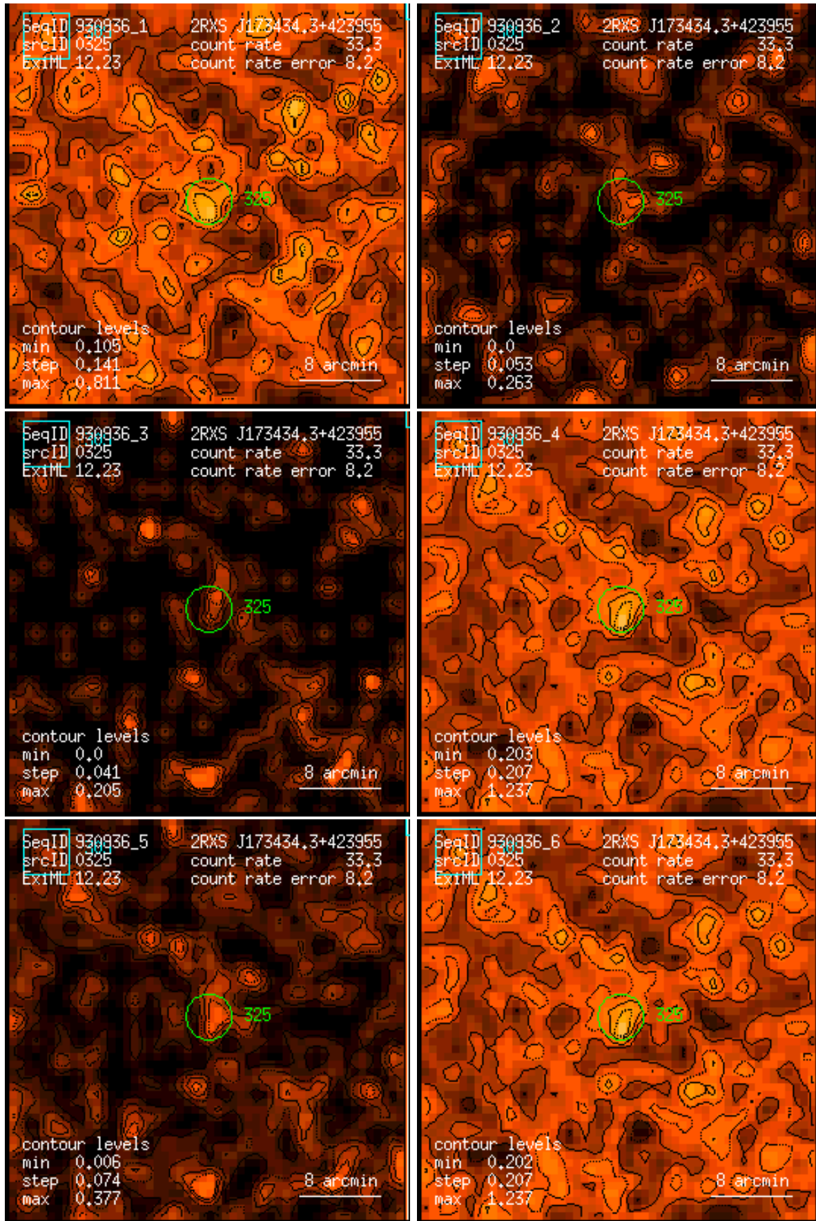
Figure 325: RASS 930936: detection 0325: band rate images, Gaussian filter: (1) PSPC channels 11 – 41, (2) 52 – 90, (3) 91 – 201, (4) 11 – 235, (5) 52 – 201, (6) 11 – 201. Broad band rates in counts/ks. Band rate contour levels in counts/ks/arcmin 2 .
