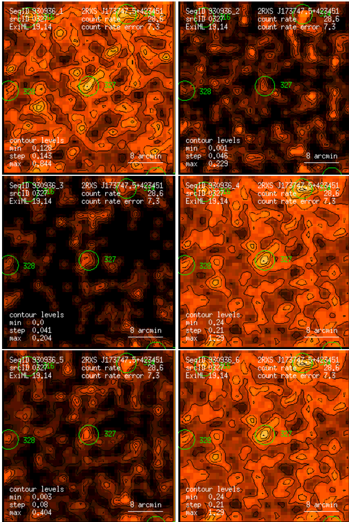
Figure 327: RASS 930936: detection 0327: band rate images, Gaussian filter: (1) PSPC channels 11 – 41, (2) 52 – 90, (3) 91 – 201, (4) 11 – 235, (5) 52 – 201, (6) 11 – 201. Broad band rates in counts/ks. Band rate contour levels in counts/ks/arcmin 2 .
