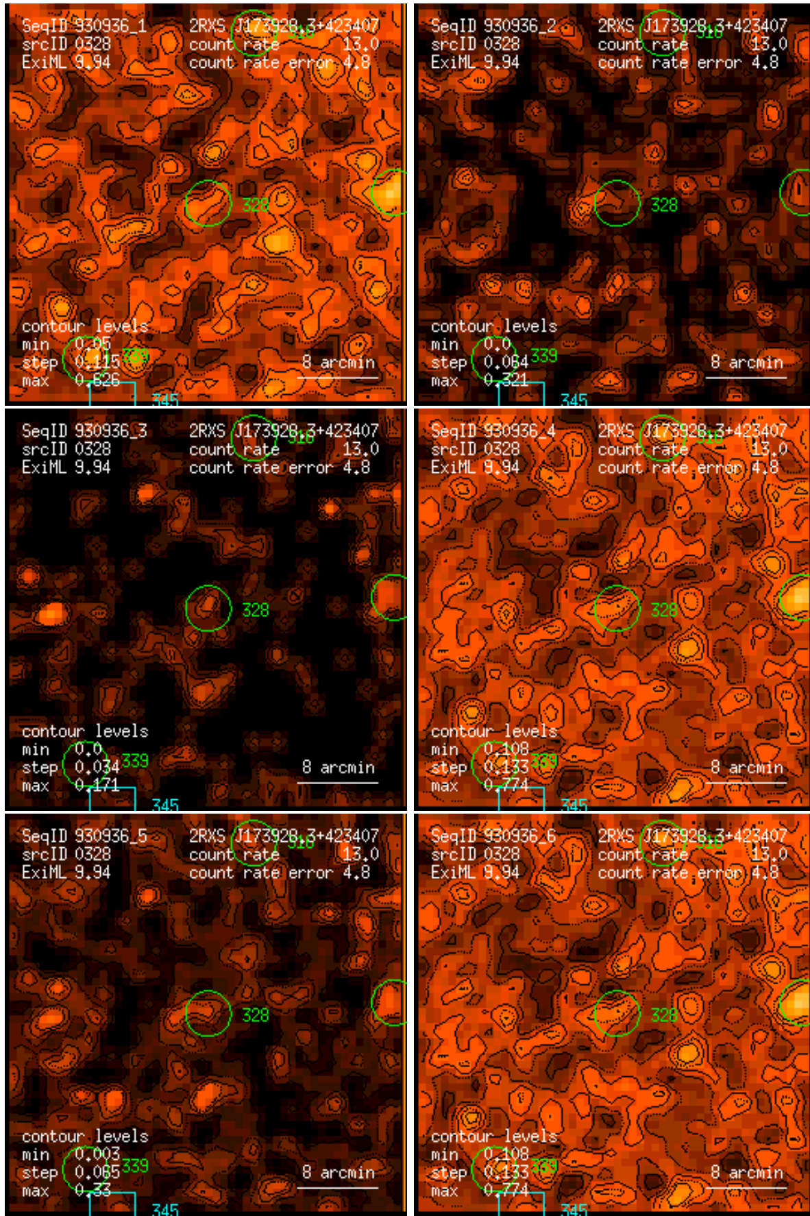
Figure 328: RASS 930936: detection 0328: band rate images, Gaussian filter: (1) PSPC channels 11 – 41, (2) 52 – 90, (3) 91 – 201, (4) 11 – 235, (5) 52 – 201, (6) 11 – 201. Broad band rates in counts/ks. Band rate contour levels in counts/ks/arcmin 2 .
