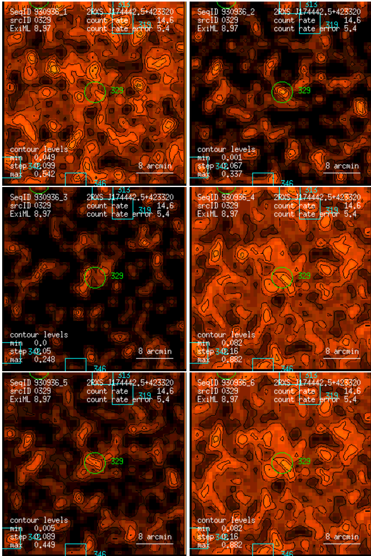
Figure 329: RASS 930936: detection 0329: band rate images, Gaussian filter: (1) PSPC channels 11 – 41, (2) 52 – 90, (3) 91 – 201, (4) 11 – 235, (5) 52 – 201, (6) 11 – 201. Broad band rates in counts/ks. Band rate contour levels in counts/ks/arcmin 2 .
