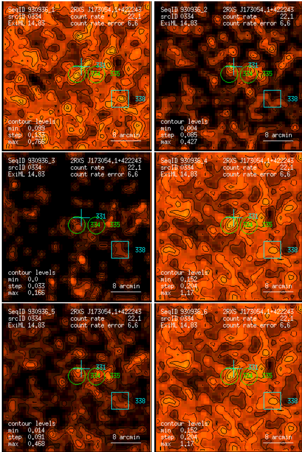
Figure 334: RASS 930936: detection 0334: band rate images, Gaussian filter: (1) PSPC channels 11 – 41, (2) 52 – 90, (3) 91 – 201, (4) 11 – 235, (5) 52 – 201, (6) 11 – 201. Broad band rates in counts/ks. Band rate contour levels in counts/ks/arcmin 2 .
