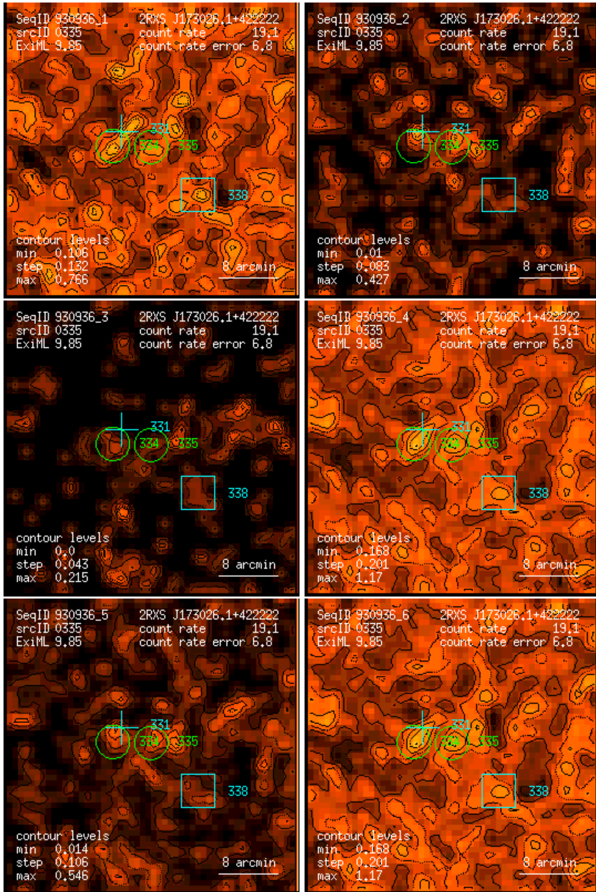
Figure 335: RASS 930936: detection 0335: band rate images, Gaussian filter: (1) PSPC channels 11 – 41, (2) 52 – 90, (3) 91 – 201, (4) 11 – 235, (5) 52 – 201, (6) 11 – 201. Broad band rates in counts/ks. Band rate contour levels in counts/ks/arcmin 2 .
