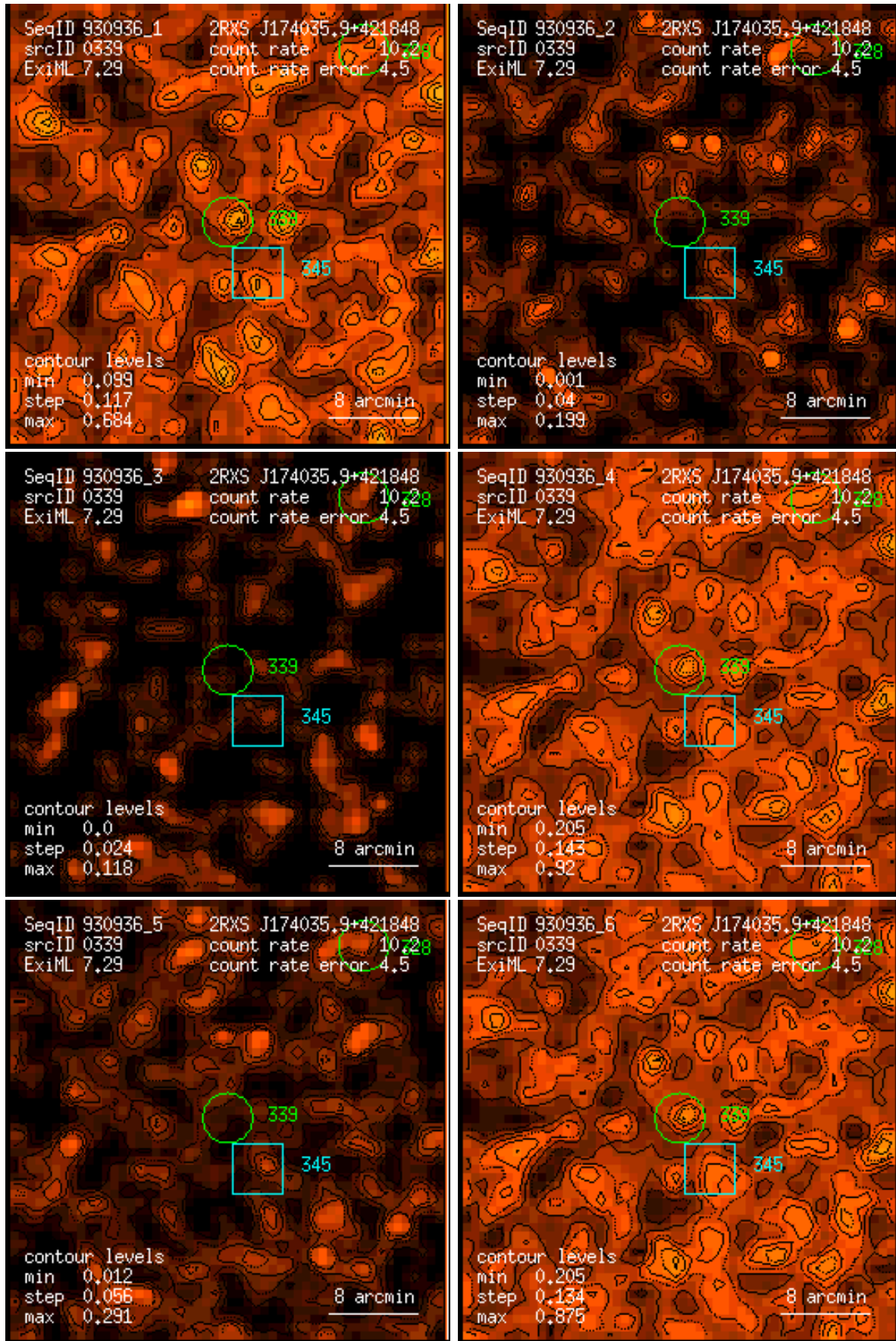
Figure 339: RASS 930936: detection 0339: band rate images, Gaussian filter: (1) PSPC channels 11 – 41, (2) 52 – 90, (3) 91 – 201, (4) 11 – 235, (5) 52 – 201, (6) 11 – 201. Broad band rates in counts/ks. Band rate contour levels in counts/ks/arcmin 2 .
