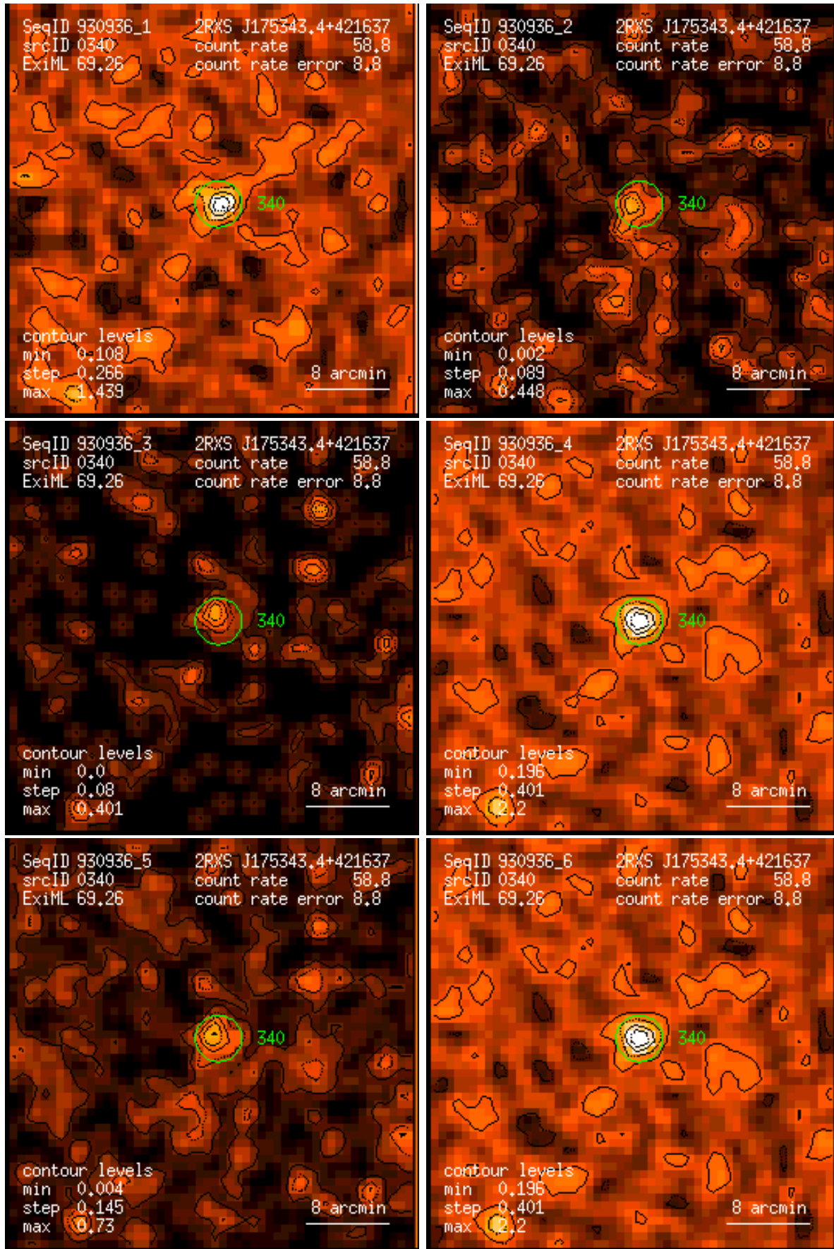
Figure 340: RASS 930936: detection 0340: band rate images, Gaussian filter: (1) PSPC channels 11 – 41, (2) 52 – 90, (3) 91 – 201, (4) 11 – 235, (5) 52 – 201, (6) 11 – 201. Broad band rates in counts/ks. Band rate contour levels in counts/ks/arcmin 2 .
